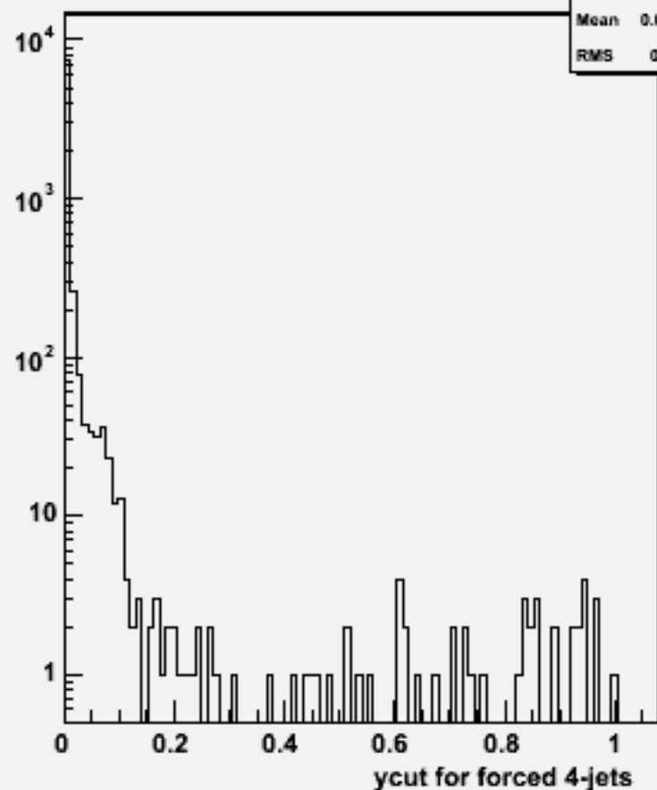
Ycut for 4-jets :w103399 e1a_e1e3e3dd_o
