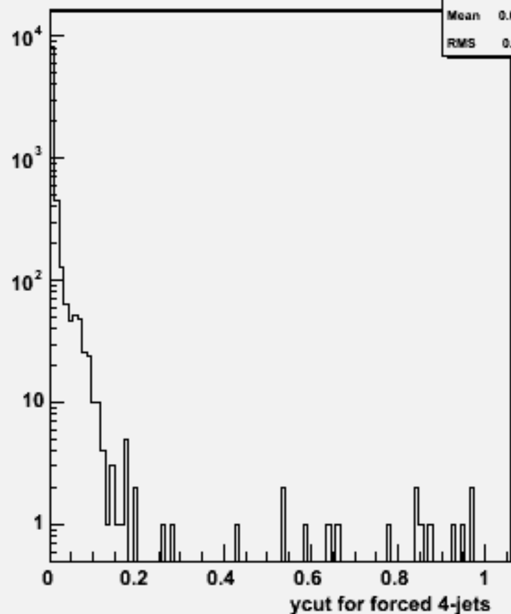
Ycut for 4-jets :w103393 e1a_e1e2e2bb_o
