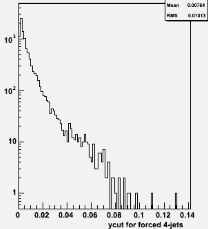
Ycut for 4-jets :w103392 e1a_e1e2e2bb_o
