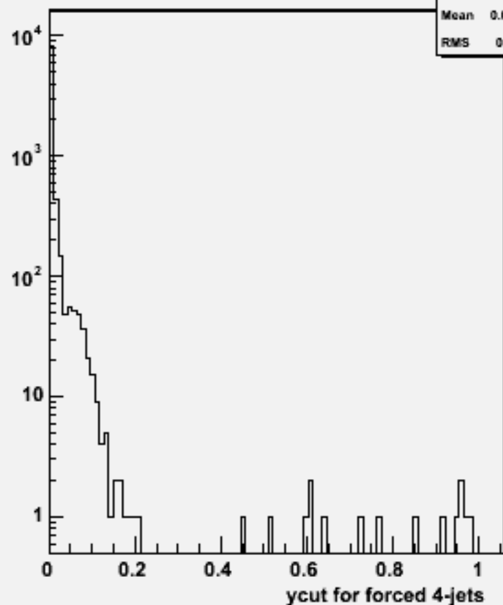
Ycut for 4-jets :w103387 e1a_e1e2e2ss_o
