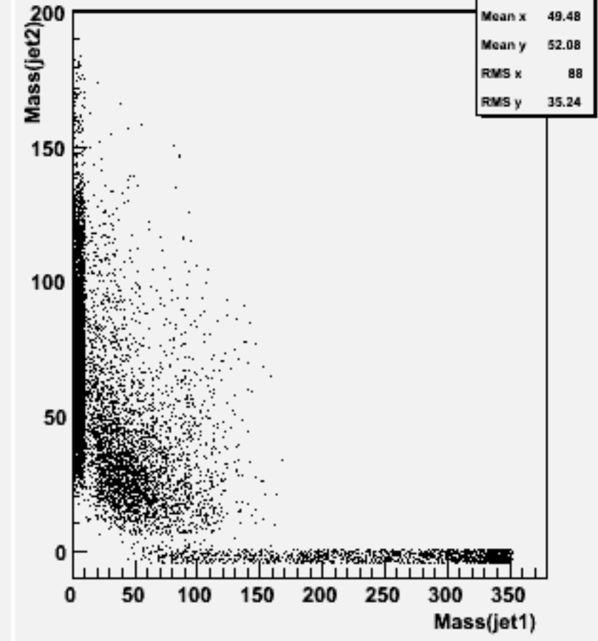
Jet mass for forced 2-jets : w103385 e1a_e1e2e2dd_o
