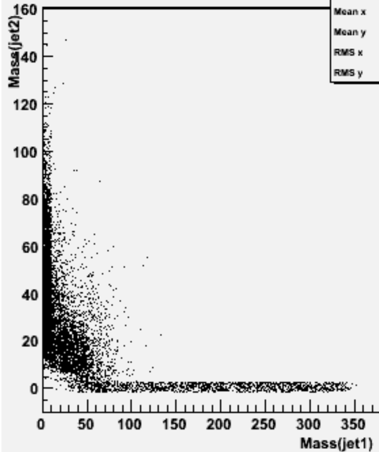
Jet mass for forced 2-jets : w103381 e1a_e1e2e2e3e3_o
