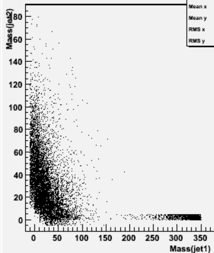
Jet mass for forced 2-jets : w103378 e1a_e1e2e2e3e3_o
