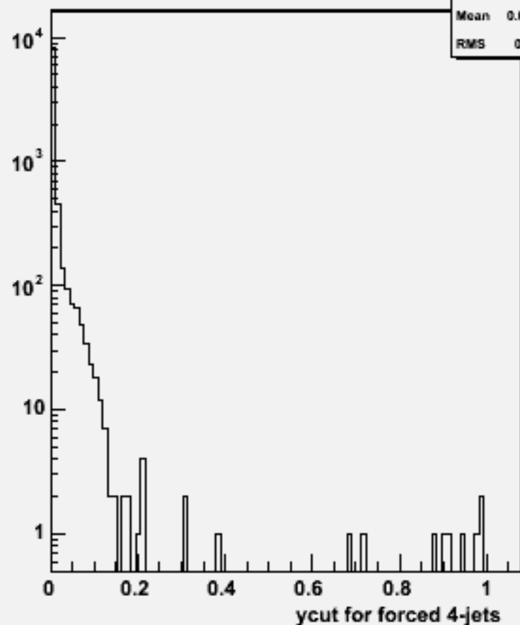
Ycut for 4-jets :w103371 e1a_e1e1e1bb_o
