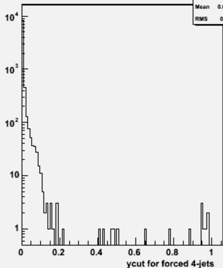
Ycut for 4-jets :w103369 e1a_e1e1e1ss_o
