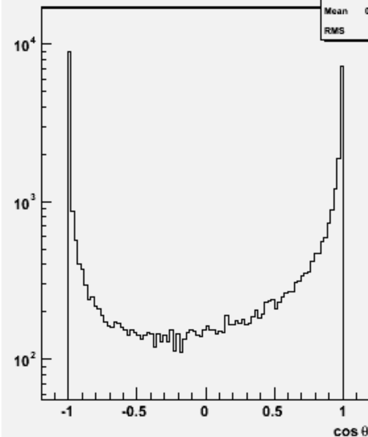
Jet cos \theta (All jets)w103366 e1a_e1e1e1ss_o
