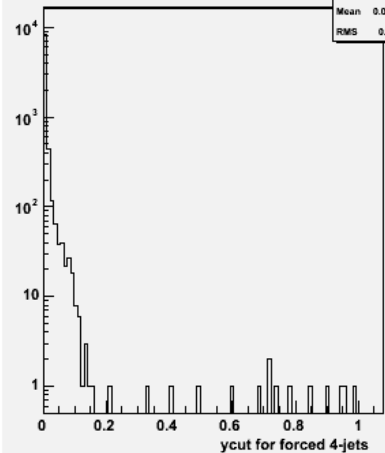
Ycut for 4-jets :w103365 e1a_e1e1e1dd_o
