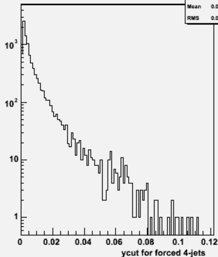
Ycut for 4-jets :w103362 e1a_e1e1e1dd_o
