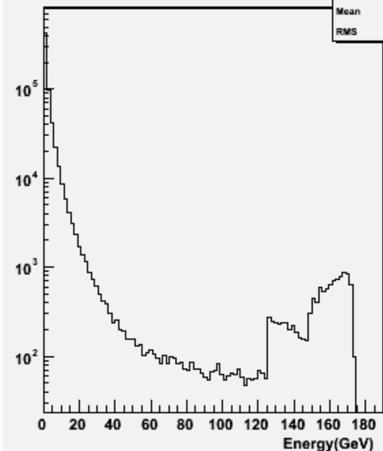
Particle Energy : w103349 e1a_e1ccbb_o
