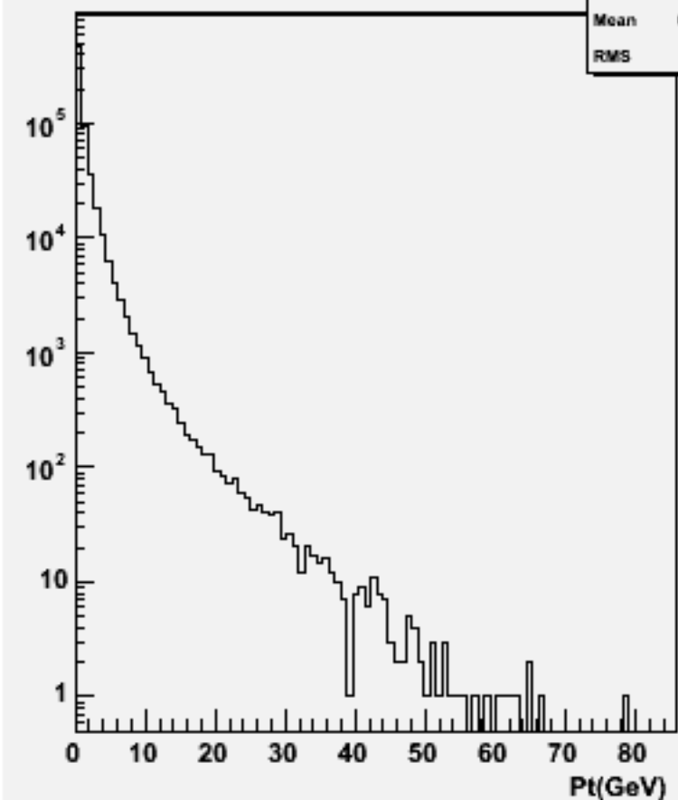
Particle Pt : w103349 e1a_e1ccbb_o
