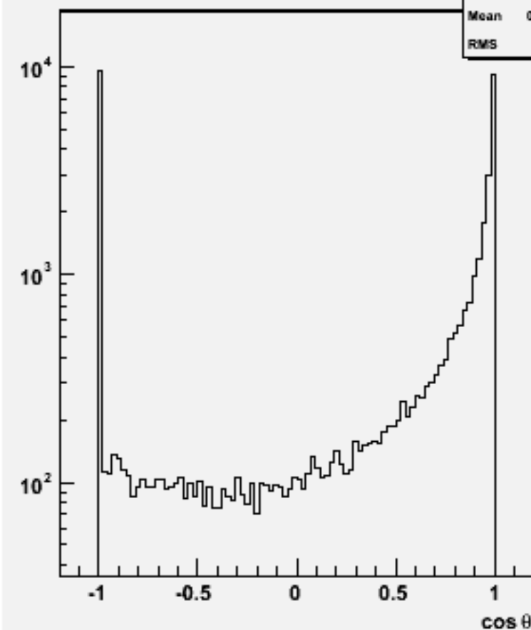
Jet cos \theta (All jets)w103349 e1a_e1ccbb_o
