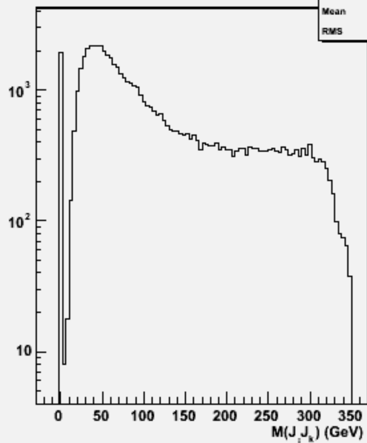
2jets mass(All comb)w103349 e1a_e1ccbb_o
