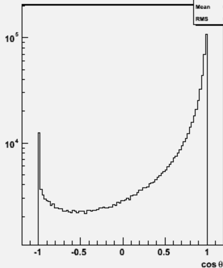
Particle cosθ : w103349 e1a_e1ccbb_o
