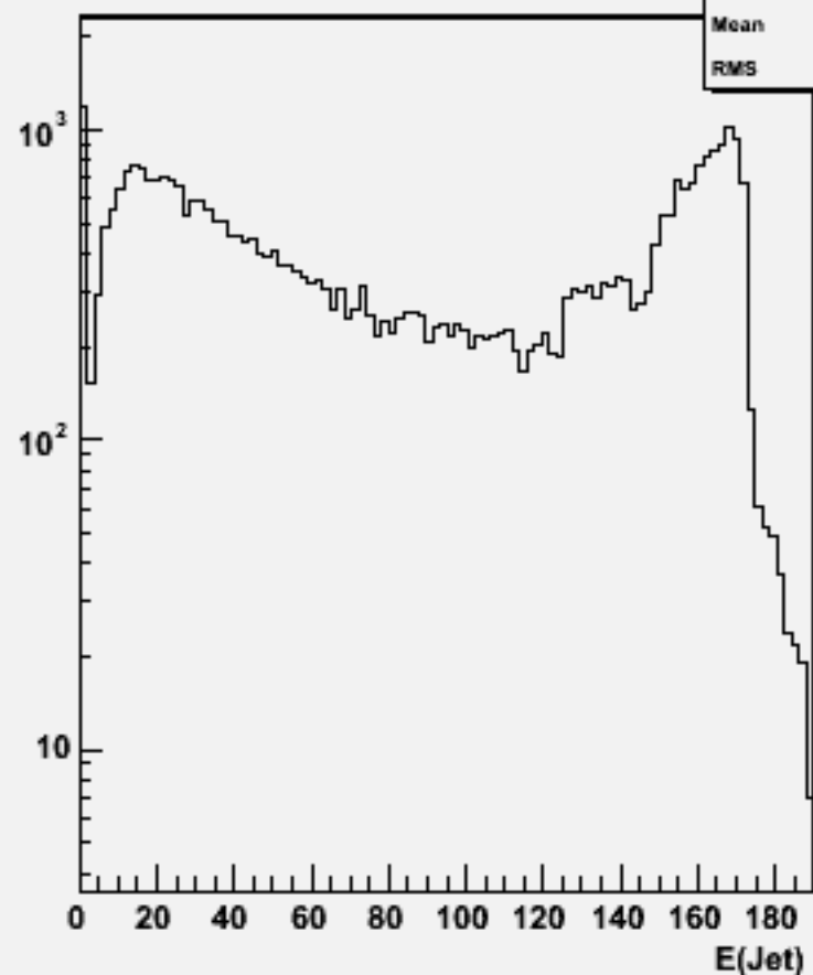
Jet energies(All jets)w103349 e1a_e1ccbb_o
