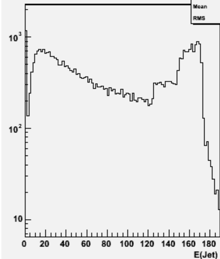
Jet energies(All jets)w103347 e1a_e1ccbb_o
