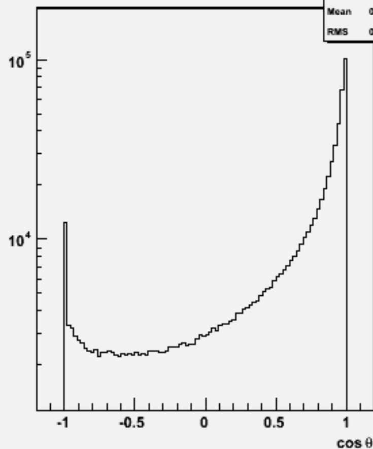
Particle cosθ : w103347 e1a_e1ccbb_o
