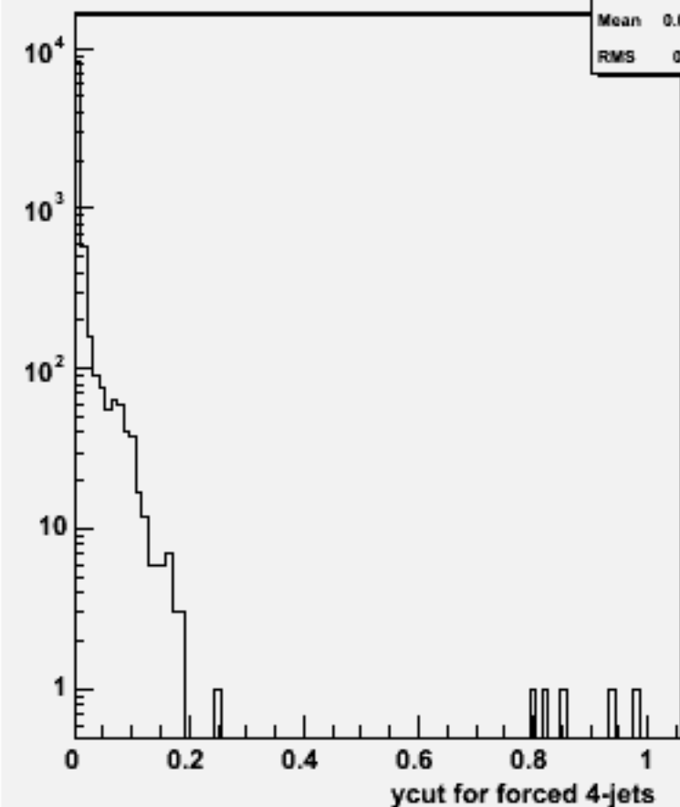
Ycut for 4-jets :w103347 e1a_e1ccbb_o
