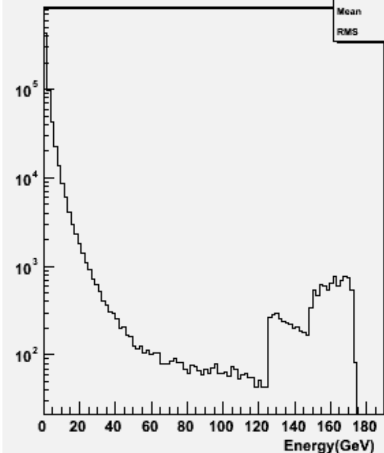
Particle Energy : w103347 e1a_e1ccbb_o
