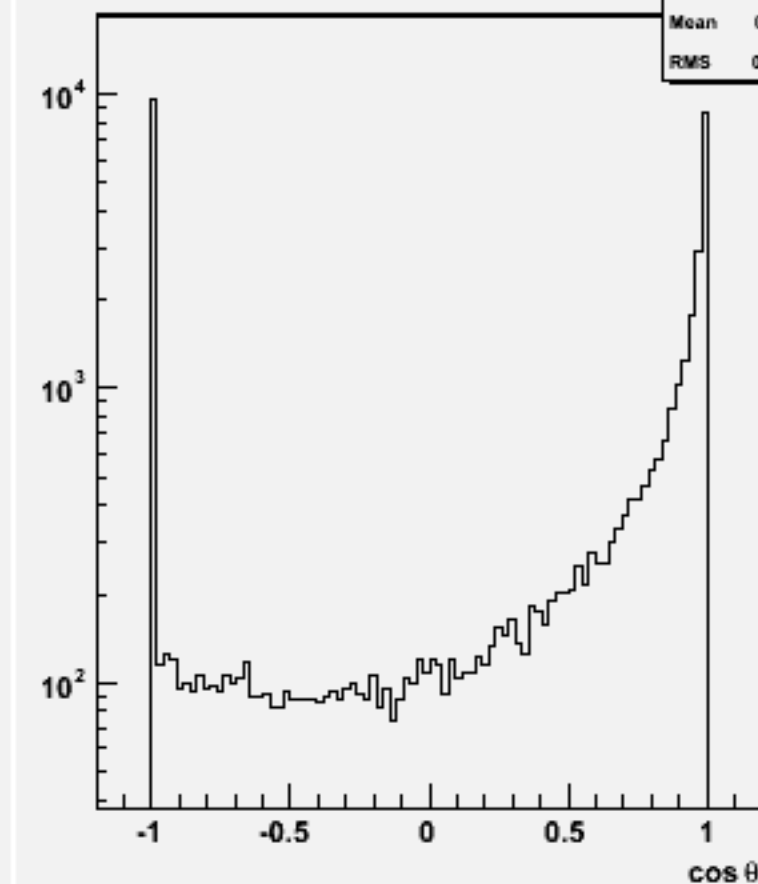
Jet cos \theta (All jets)w103347 e1a_e1ccbb_o
