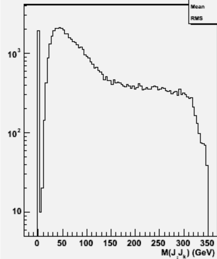
2jets mass(All comb)w103347 e1a_e1ccbb_o
