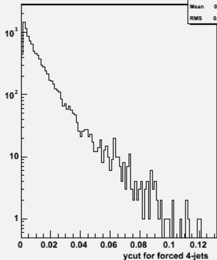
Ycut for 4-jets :w103346 e1a_e1ccbb_o
