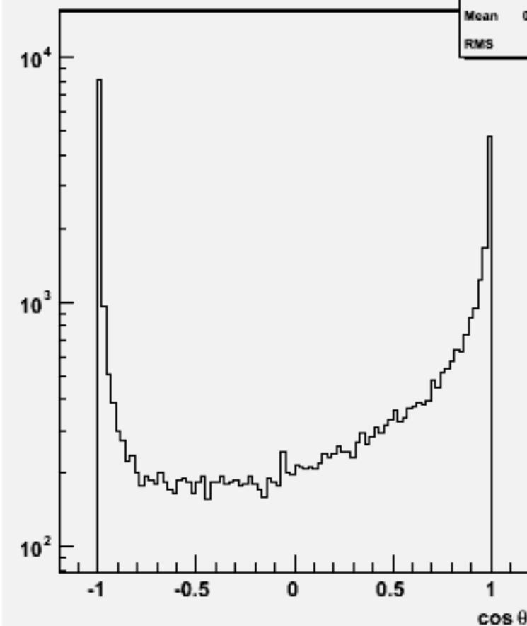
Jet cos \theta (All jets)w103346 e1a_e1ccbb_o
