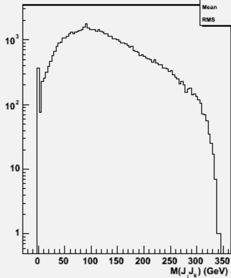
2jets mass(All comb)w103346 e1a_e1ccbb_o
