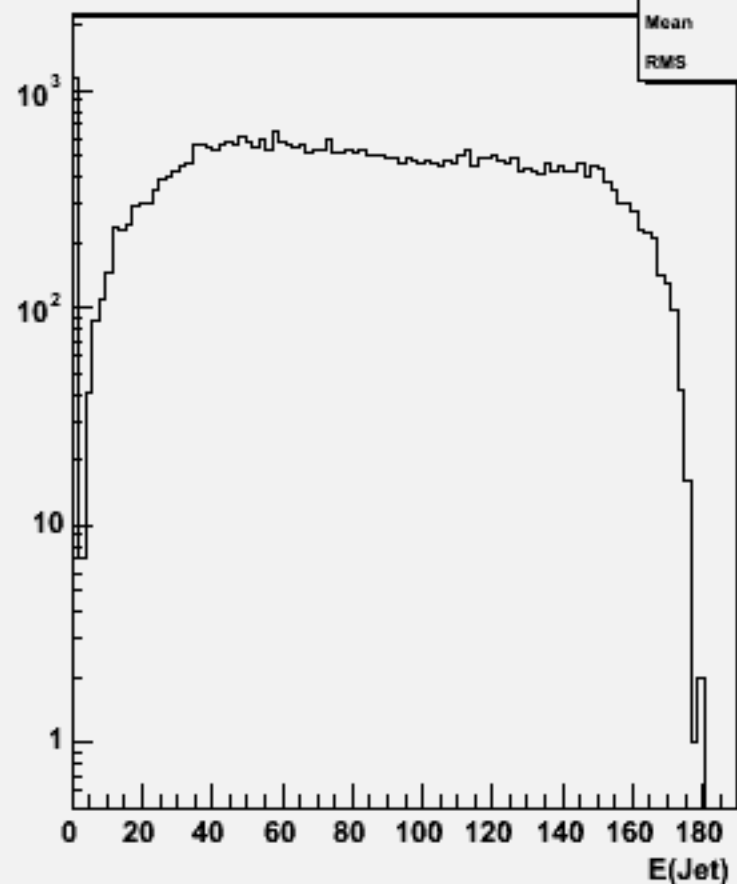
Jet energies(All jets)w103346 e1a_e1ccbb_o
