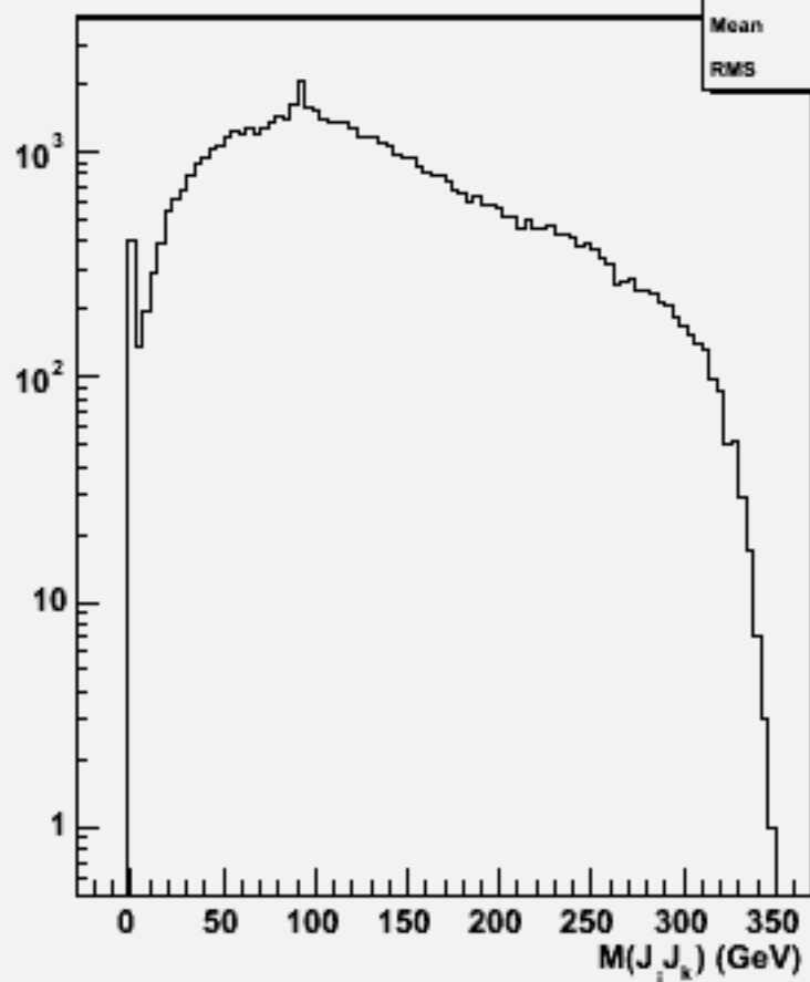
2jets mass(All comb)w103344 e1a_e1ccdd_o
