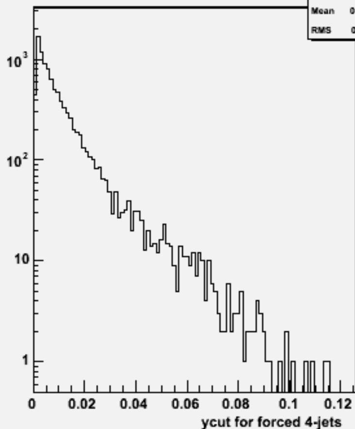
Ycut for 4-jets :w103344 e1a_e1ccdd_o
