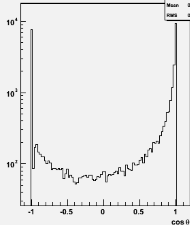
Jet cos \theta (All jets)w103341 e1a_e1cce3e3_o
