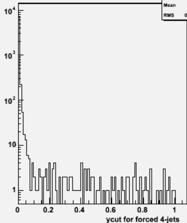
Ycut for 4-jets :w103341 e1a_e1cce3e3_o
