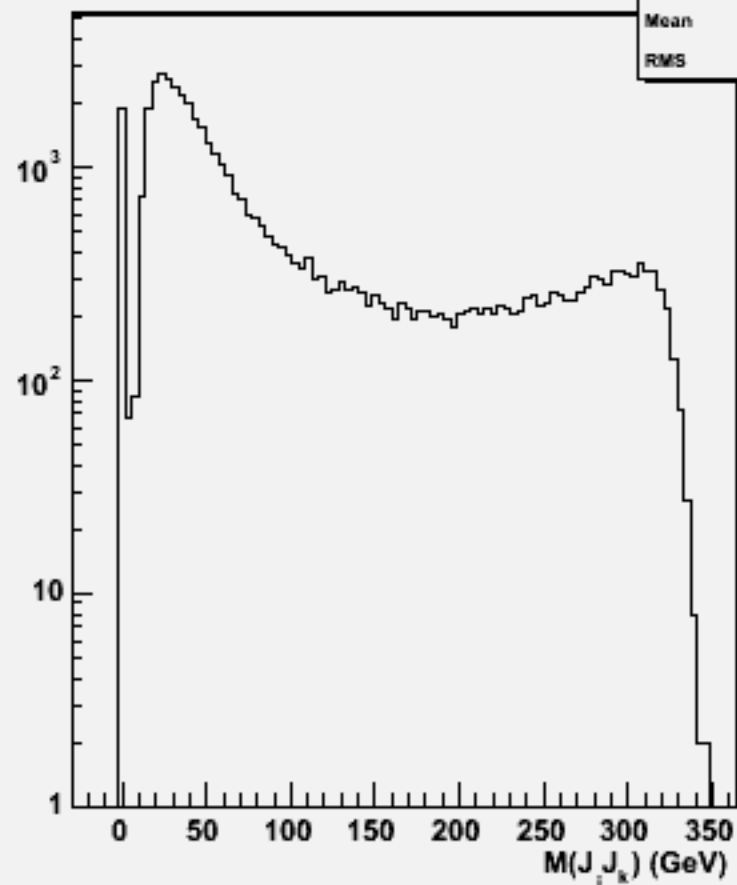
2jets mass(All comb)w103341 e1a_e1cce3e3_o
