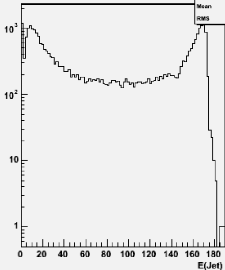
Jet energies(All jets)w103341 e1a_e1cce3e3_o
