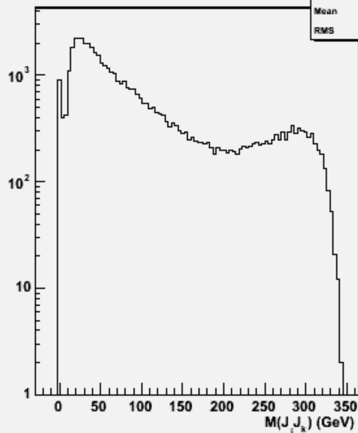
2jets mass(All comb)w103340 e1a_e1cce3e3_o
