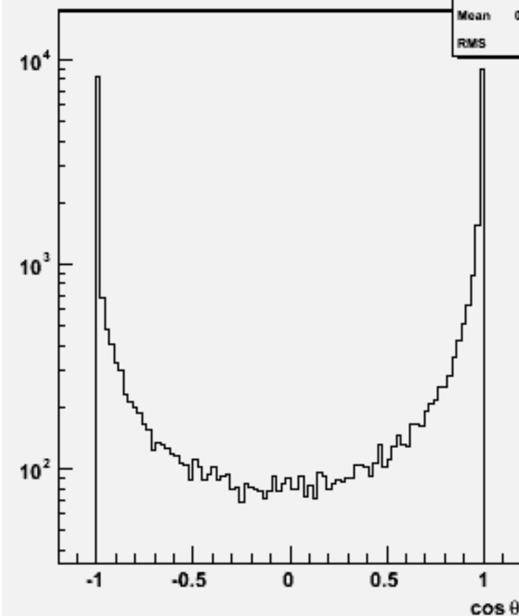
Jet cos \theta (All jets)w103340 e1a_e1cce3e3_o
