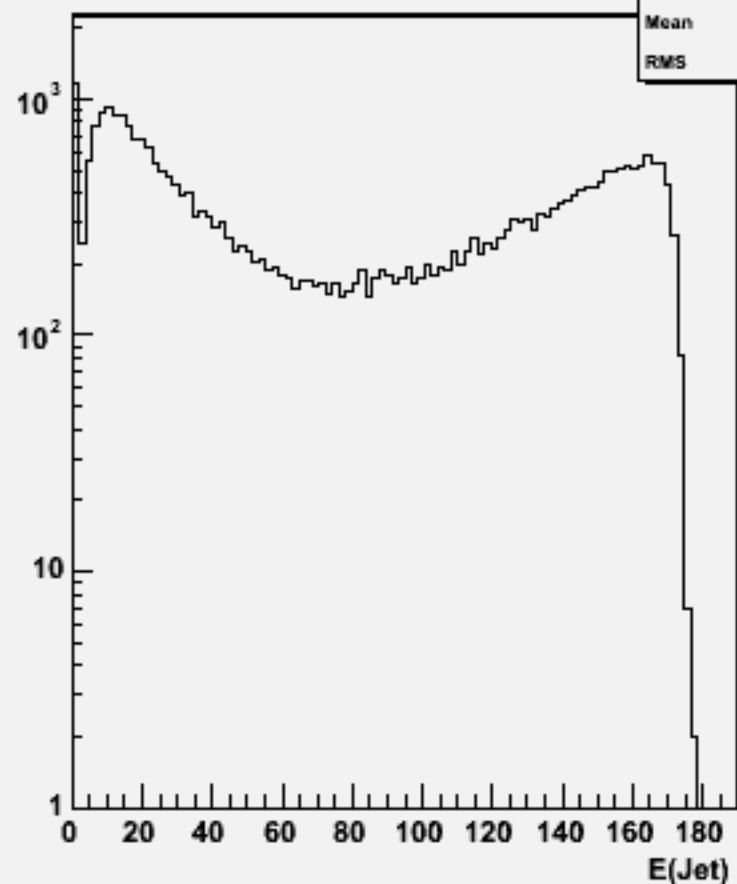
Jet energies(All jets)w103340 e1a_e1cce3e3_o
