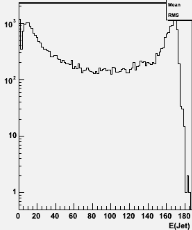
Jet energies(All jets)w103339 e1a_e1cce3e3_o
