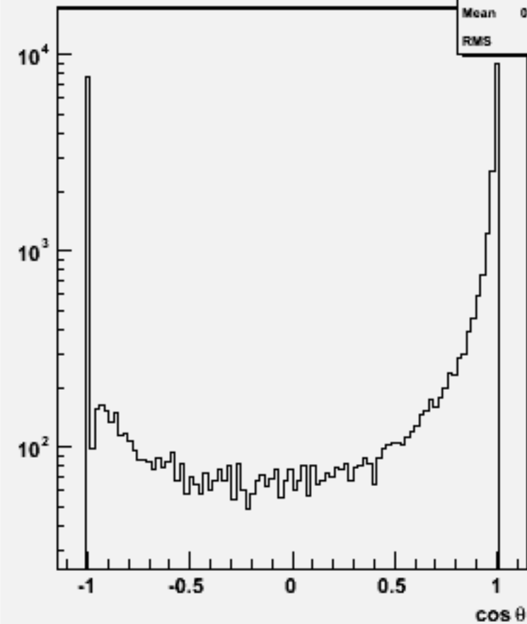
Jet cos \theta (All jets)w103339 e1a_e1cce3e3_o
