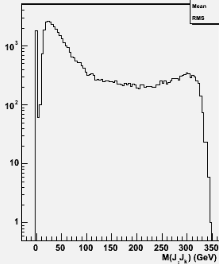
2jets mass(All comb)w103339 e1a_e1cce3e3_o
