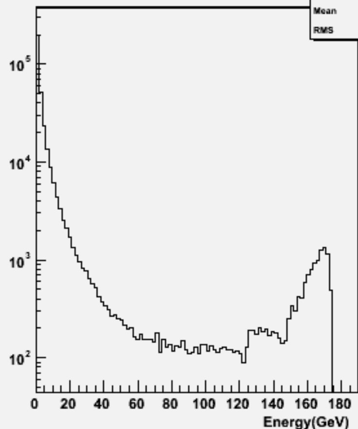
Particle Energy : w103339 e1a_e1cce3e3_o
