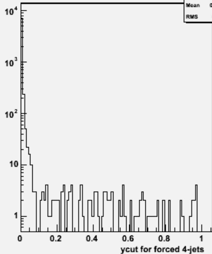
Ycut for 4-jets :w103339 e1a_e1cce3e3_o
