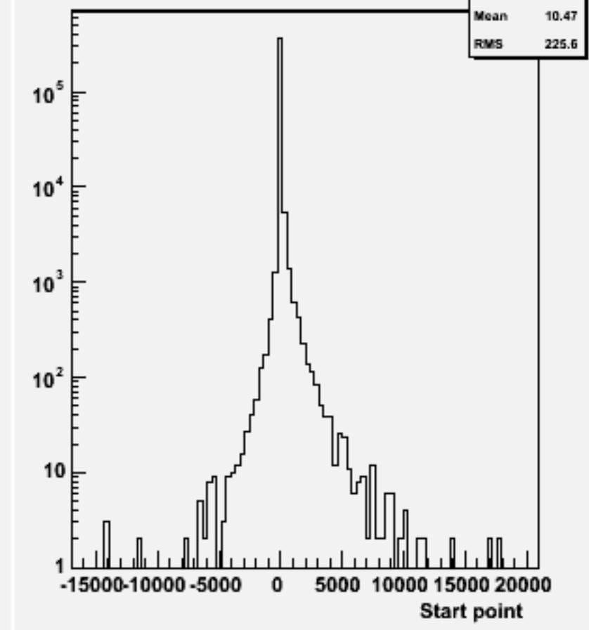
Start point Z : w103338 e1a_e1cce3e3_o
