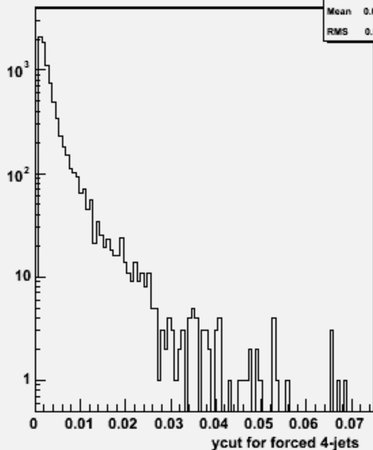
Ycut for 4-jets :w103338 e1a_e1cce3e3_o
