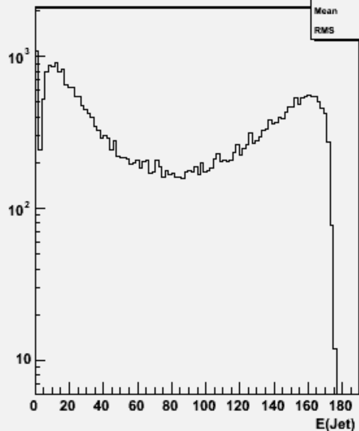
Jet energies(All jets)w103338 e1a_e1cce3e3_o
