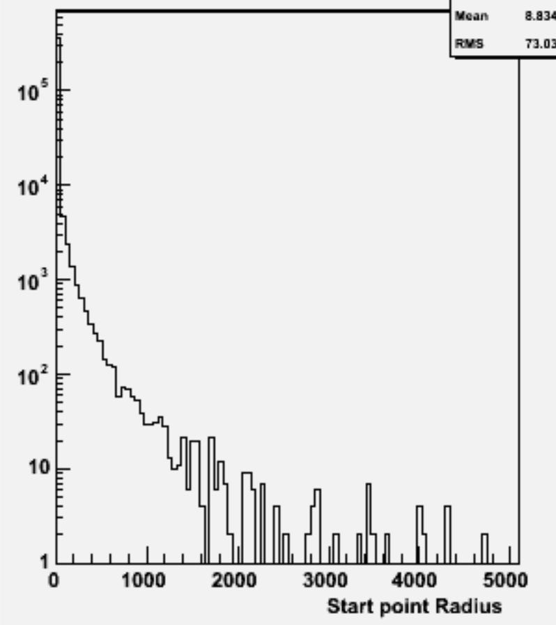
Start point R : w103338 e1a_e1cce3e3_o
