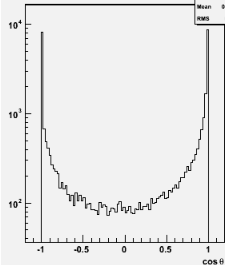
Jet cos \theta (All jets)w103338 e1a_e1cce3e3_o
