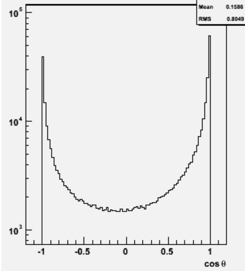
Particle cos θ : w103338 e1a_e1cce3e3_o
