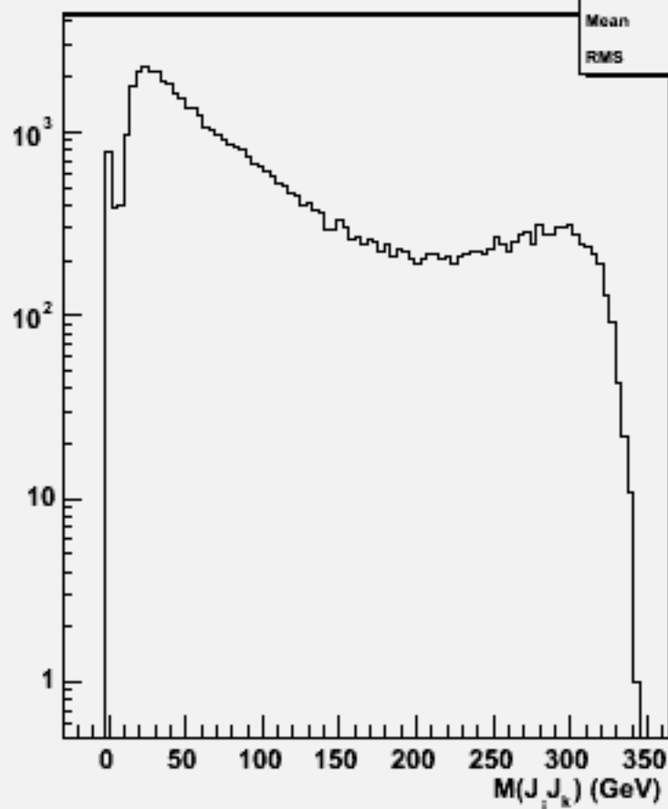
2jets mass(All comb)w103338 e1a_e1cce3e3_o
