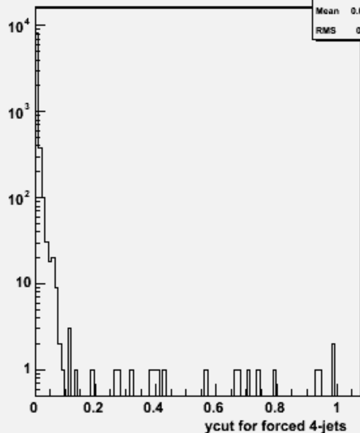
Ycut for 4-jets :w103337 e1a_e1cce2e2_o
