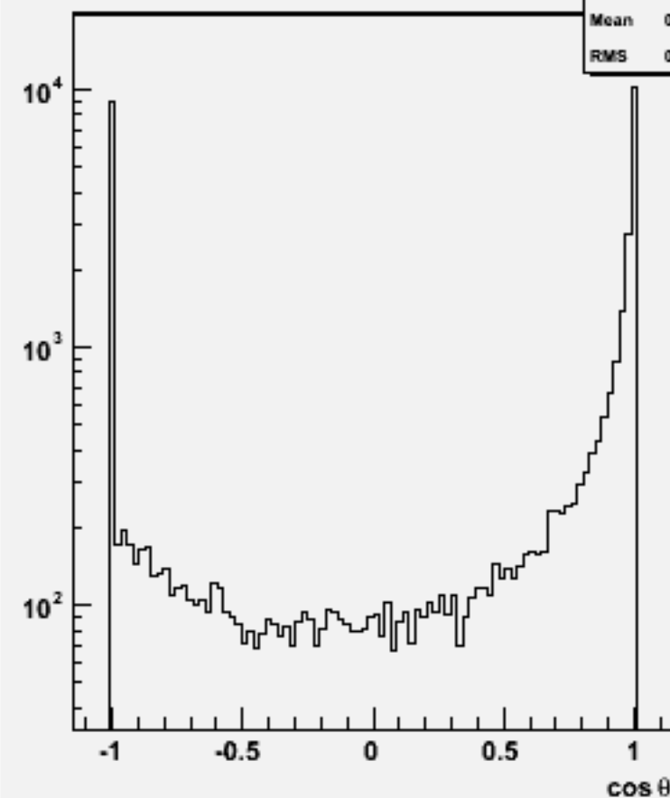
Jet cos \theta (All jets)w103337 e1a_e1cce2e2_o
