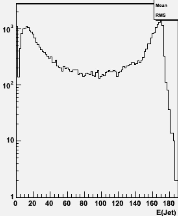
Jet energies(All jets)w103337 e1a_e1cce2e2_o
