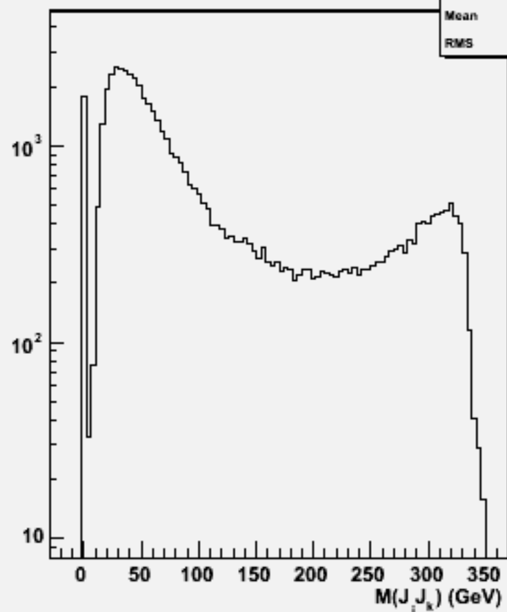
2jets mass(All comb)w103337 e1a_e1cce2e2_o
