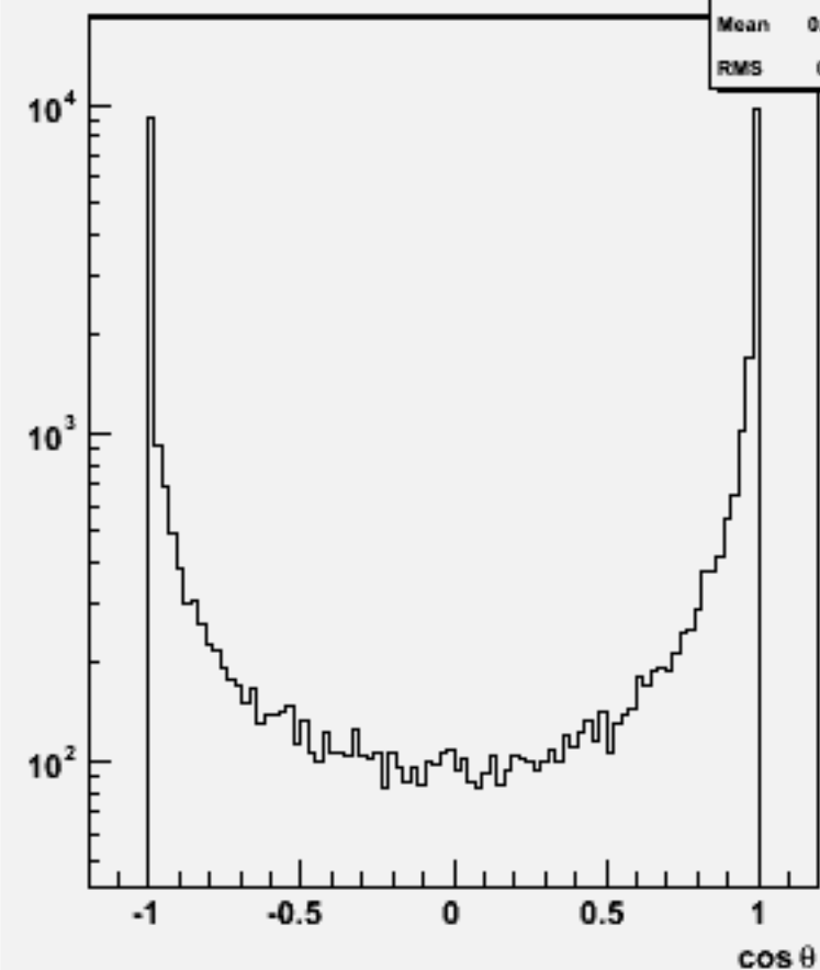
Jet cos \theta (All jets)w103336 e1a_e1cce2e2_o
