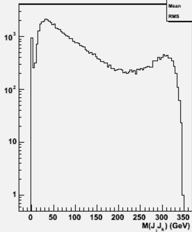
2jets mass(All comb)w103336 e1a_e1cce2e2_o
