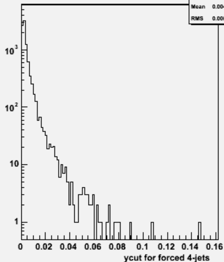
Ycut for 4-jets :w103336 e1a_e1cce2e2_o
