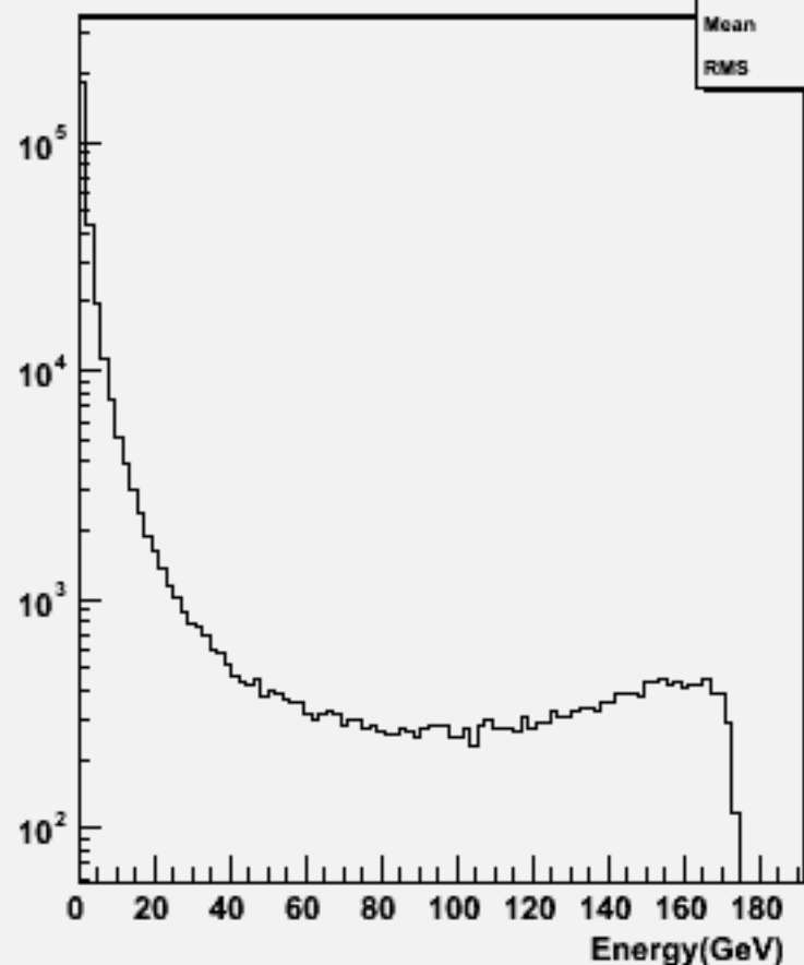
Particle Energy : w103336 e1a_e1cce2e2_o
