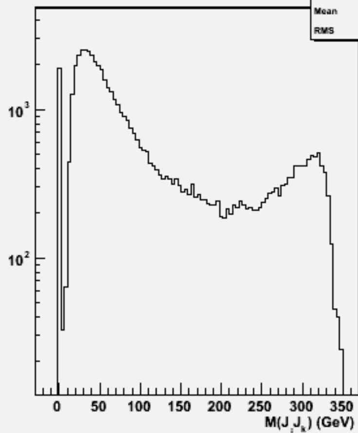
2jets mass(All comb)w103335 e1a_e1cce2e2_o
