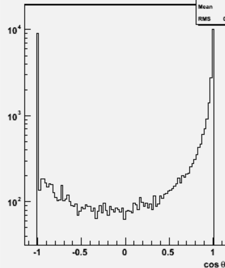
Jet cos \theta (All jets)w103335 e1a_e1cce2e2_o
