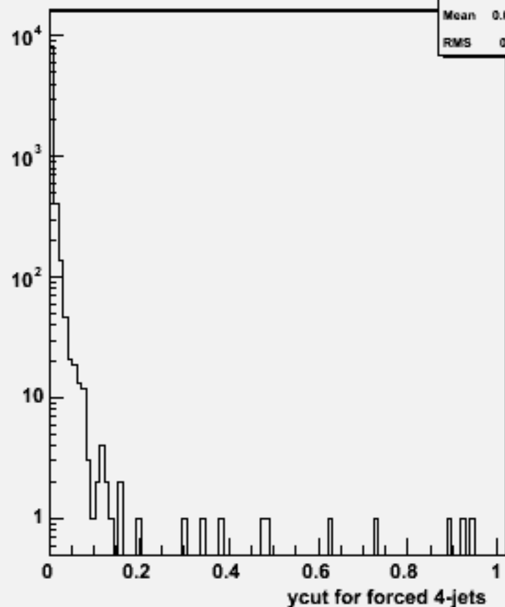
Ycut for 4-jets :w103335 e1a_e1cce2e2_o
