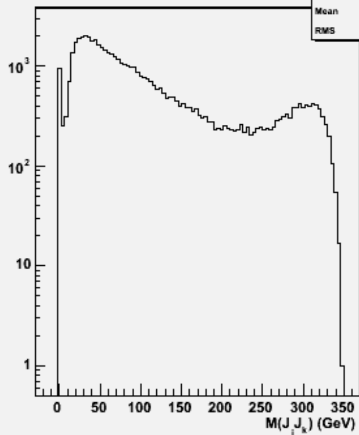
2jets mass(All comb)w103334 e1a_e1cce2e2_o
