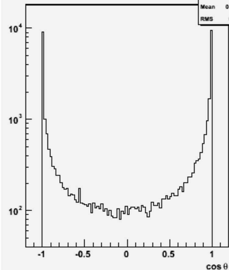
Jet cos \theta (All jets)w103334 e1a_e1cce2e2_o
