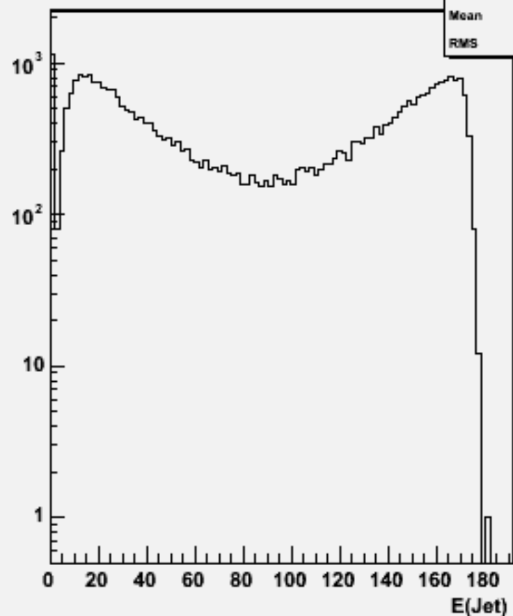
Jet energies(All jets)w103334 e1a_e1cce2e2_o
