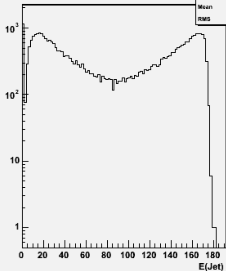
Jet energies(All jets)w103332 e1a_e1cce1e1_o
