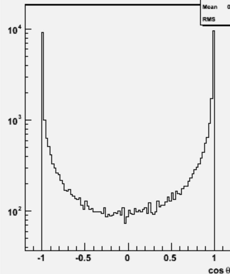
Jet cos \theta (All jets)w103332 e1a_e1cce1e1_o
