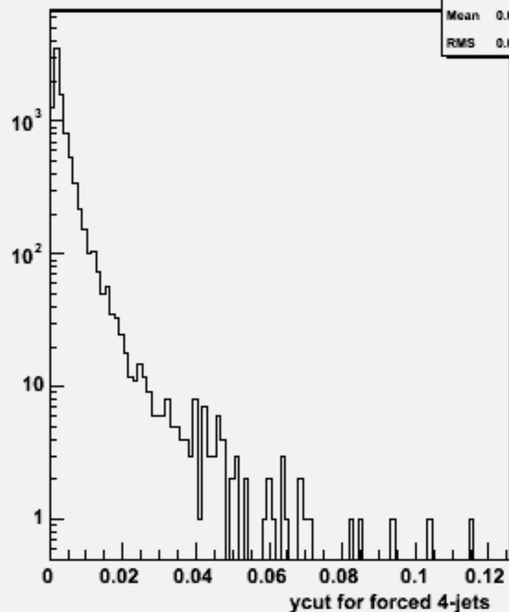
Ycut for 4-jets :w103332 e1a_e1cce1e1_o
