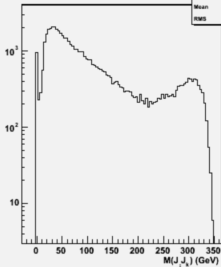
2jets mass(All comb)w103332 e1a_e1cce1e1_o
