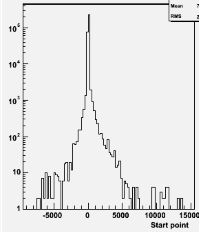
Start point Z : w103332 e1a_e1cce1e1_o
