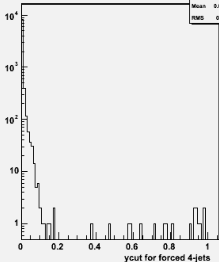
Ycut for 4-jets :w103331 e1a_e1cce1e1_o
