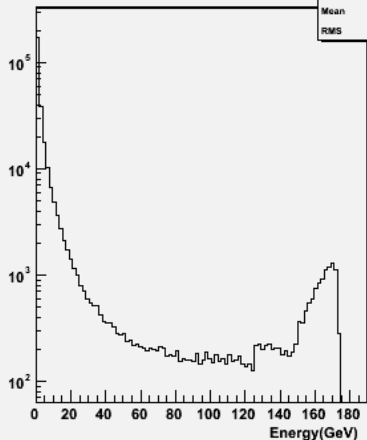
Particle Energy : w103331 e1a_e1cce1e1_o
