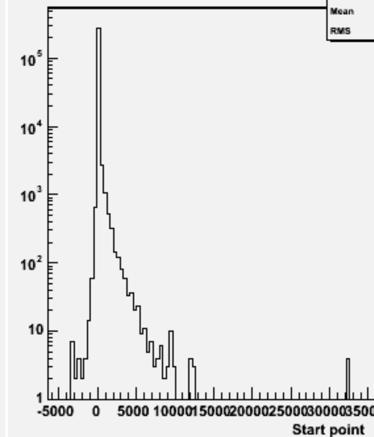
Start point Z : w103331 e1a_e1cce1e1_o
