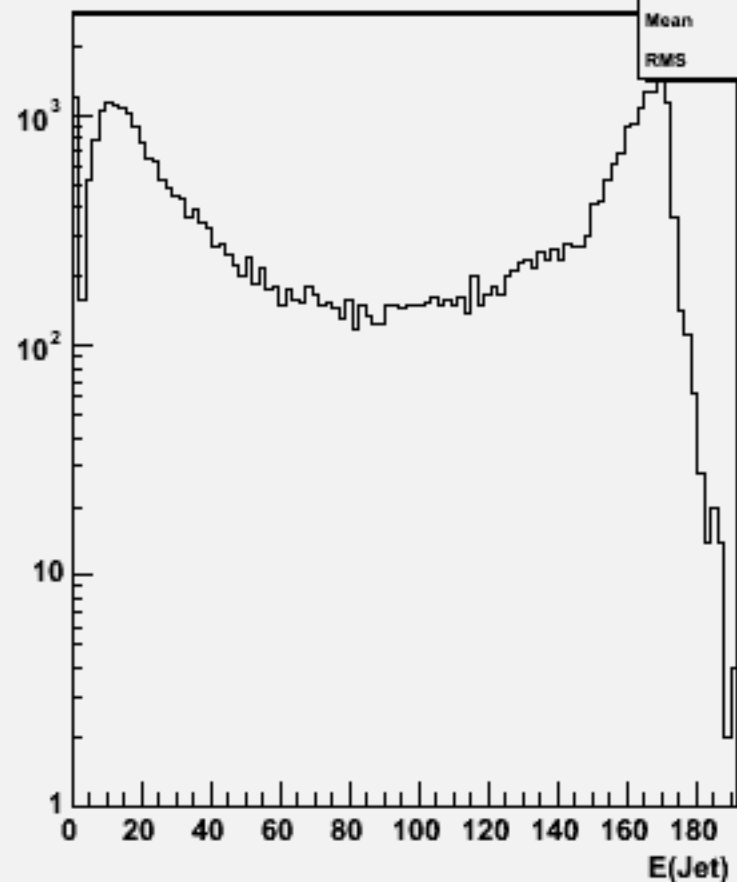
Jet energies(All jets)w103331 e1a_e1cce1e1_o
