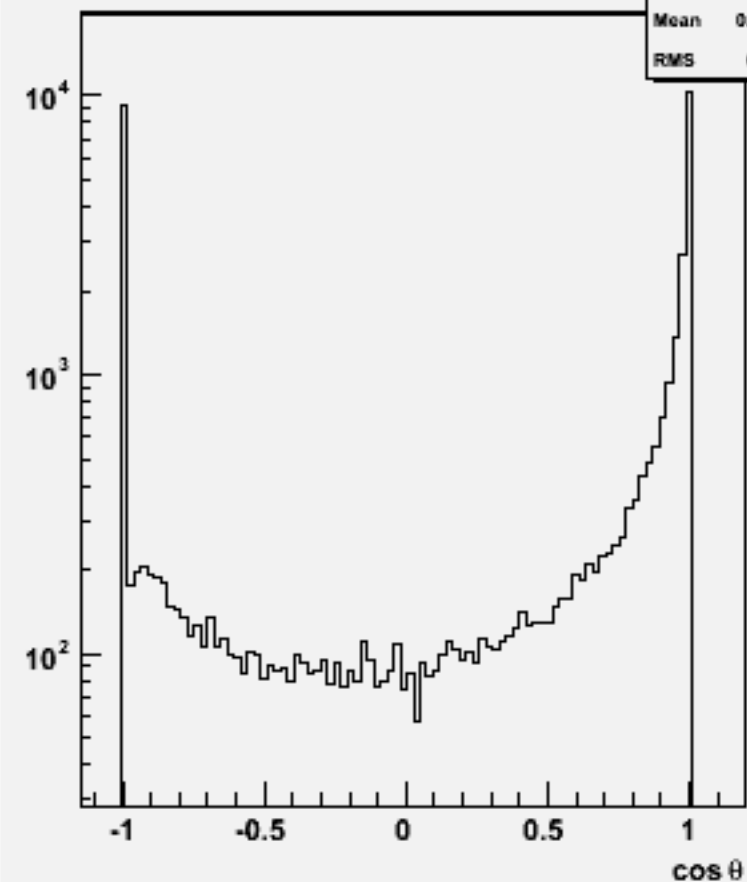
Jet cos \theta (All jets)w103331 e1a_e1cce1e1_o
