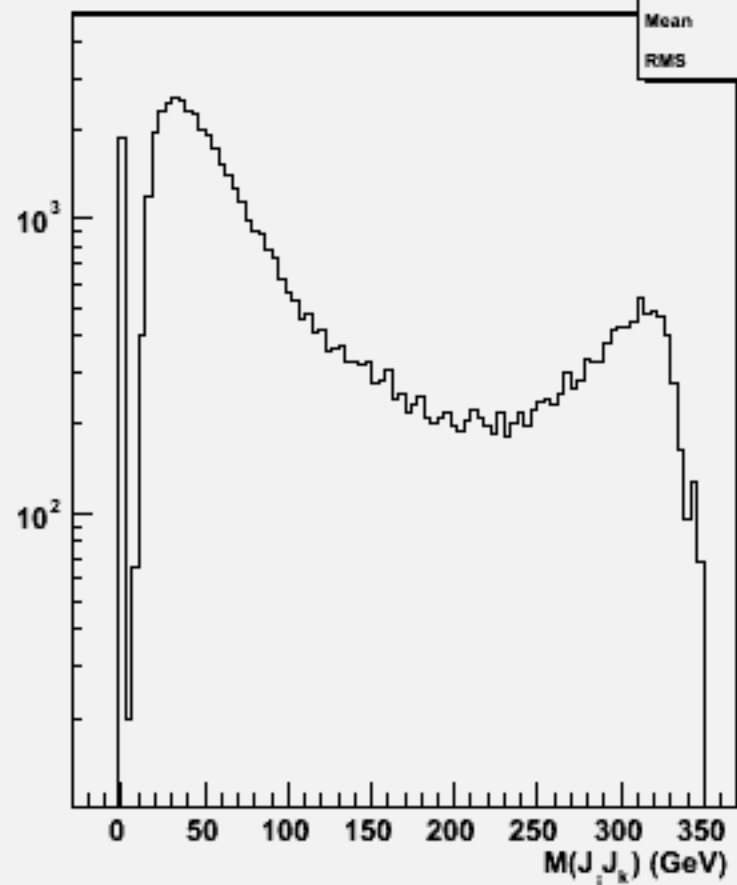
2jets mass(All comb)w103331 e1a_e1cce1e1_o
