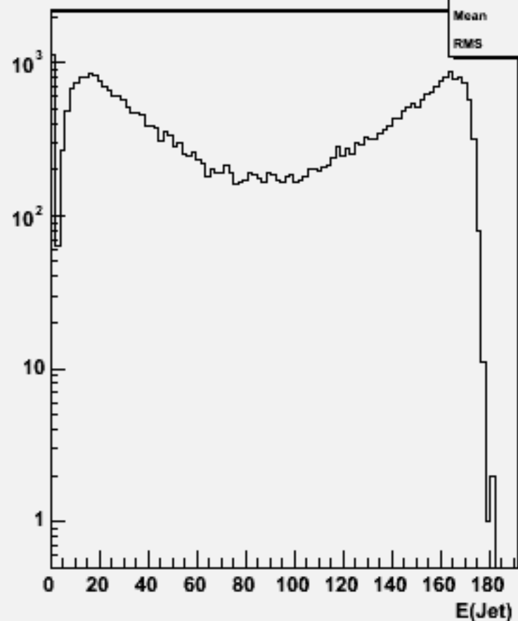
Jet energies(All jets)w103330 e1a_e1cce1e1_o
