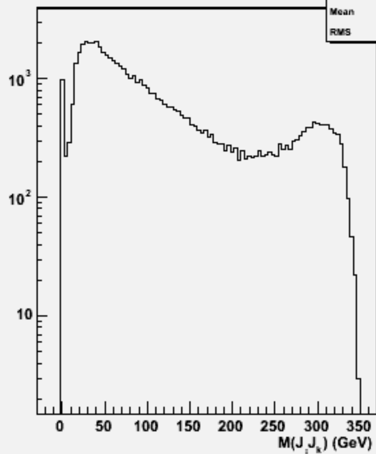
2jets mass(All comb)w103330 e1a_e1cce1e1_o
