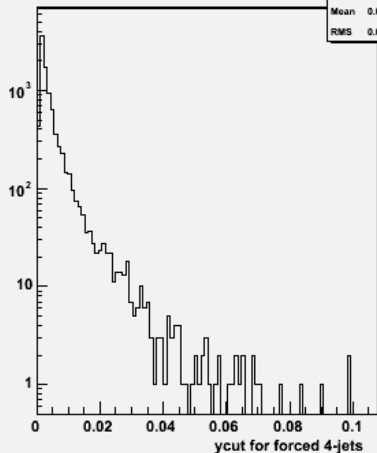
Ycut for 4-jets :w103330 e1a_e1cce1e1_o
