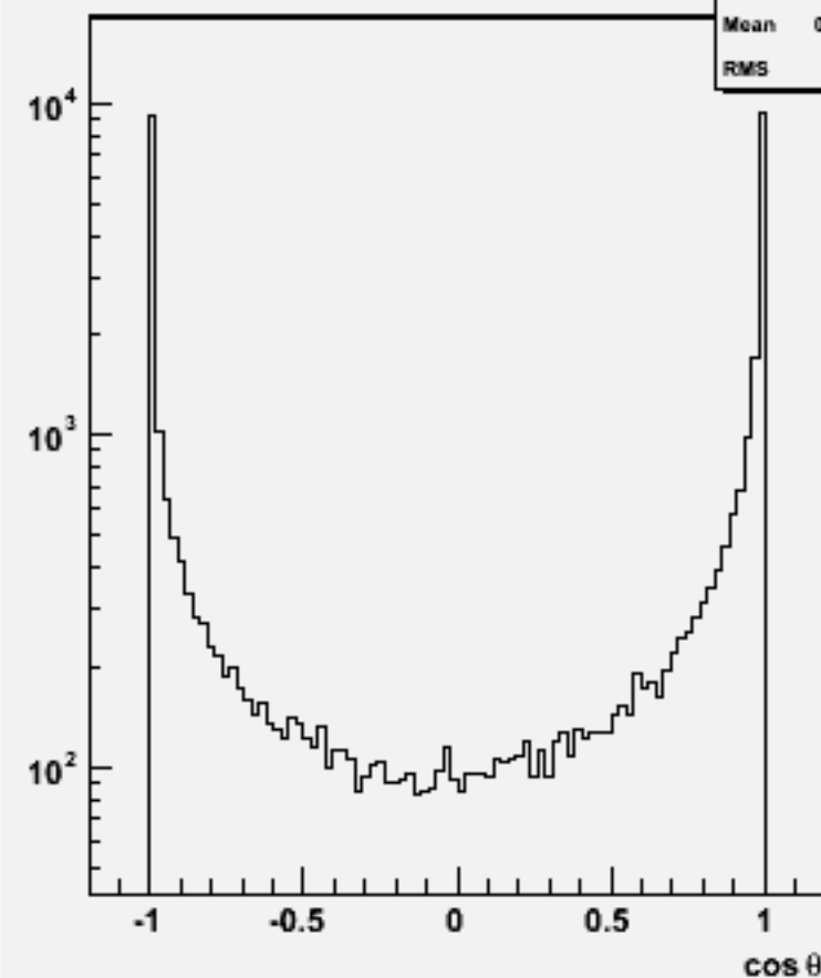
Jet cos \theta (All jets)w103330 e1a_e1cce1e1_o
