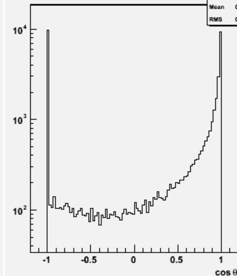
Jet cos \theta (All jets)w103329 e1a_e1uubb_o
