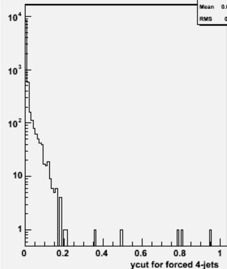
Ycut for 4-jets :w103329 e1a_e1uubb_o
