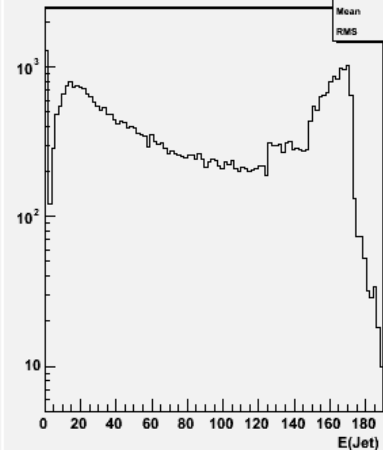
Jet energies(All jets)w103329 e1a_e1uubb_o
