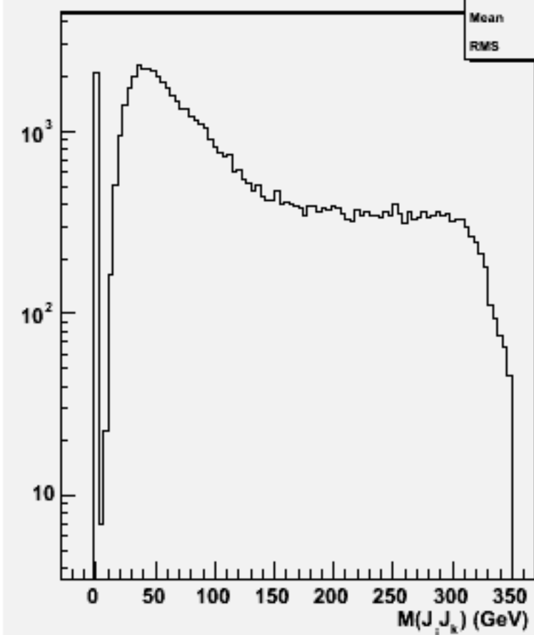
2jets mass(All comb)w103329 e1a_e1uubb_o
