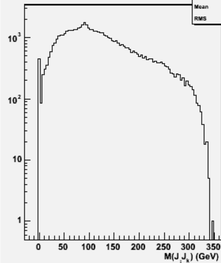
2jets mass(All comb)w103328 e1a_e1uubb_o
