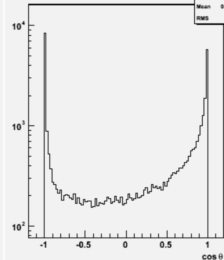
Jet cos \theta (All jets)w103328 e1a_e1uubb_o
