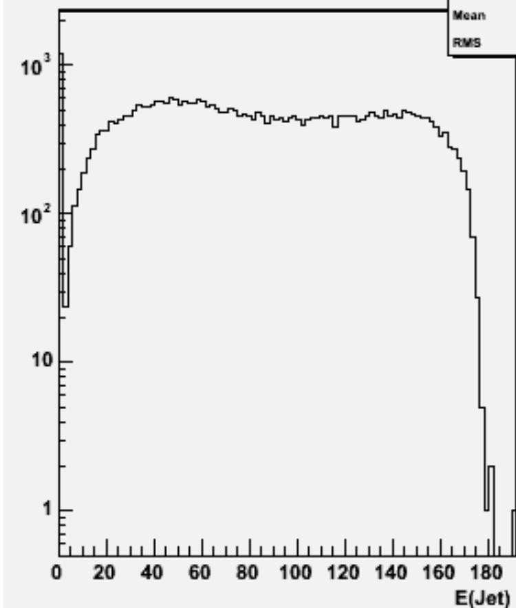
Jet energies(All jets)w103328 e1a_e1uubb_o
