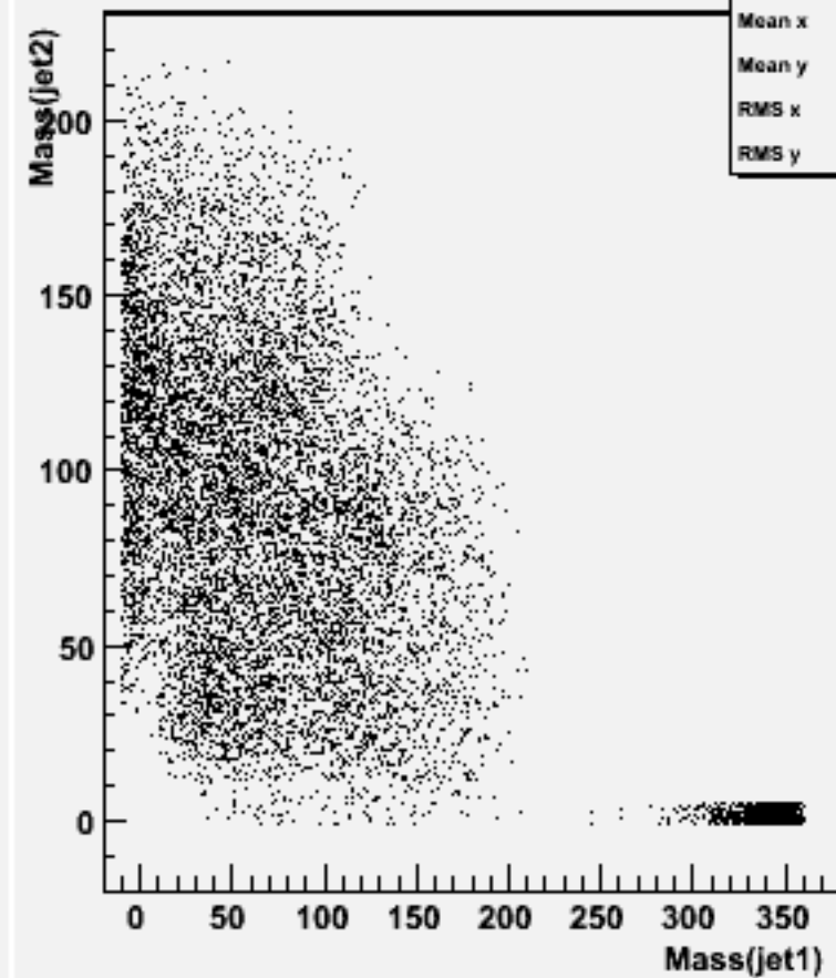
Jet mass for forced 2-jets : w103328 e1a_e1uubb_o
