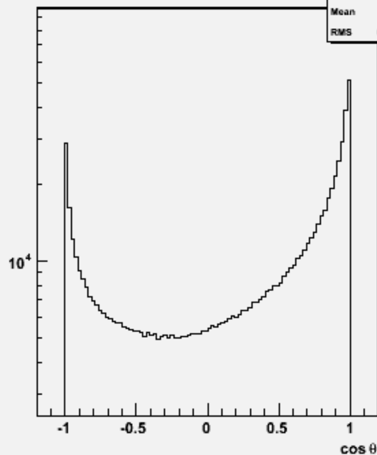
Particle cos \theta : w103328 e1a_e1uubb_o
