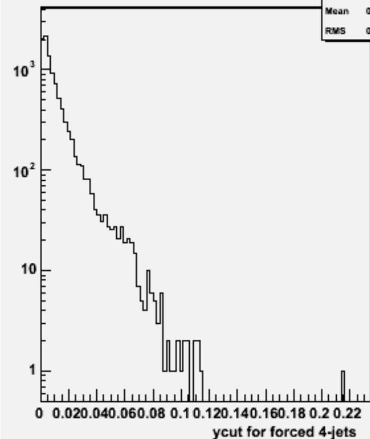
Ycut for 4-jets :w103328 e1a_e1uubb_o
