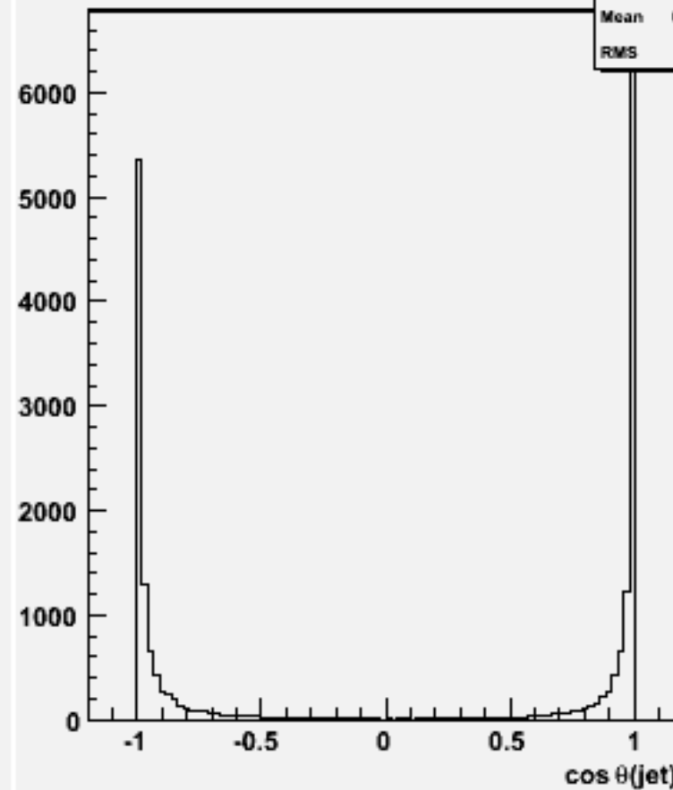
cos \theta for 2-jets :w103328 e1a_e1uubb_o
