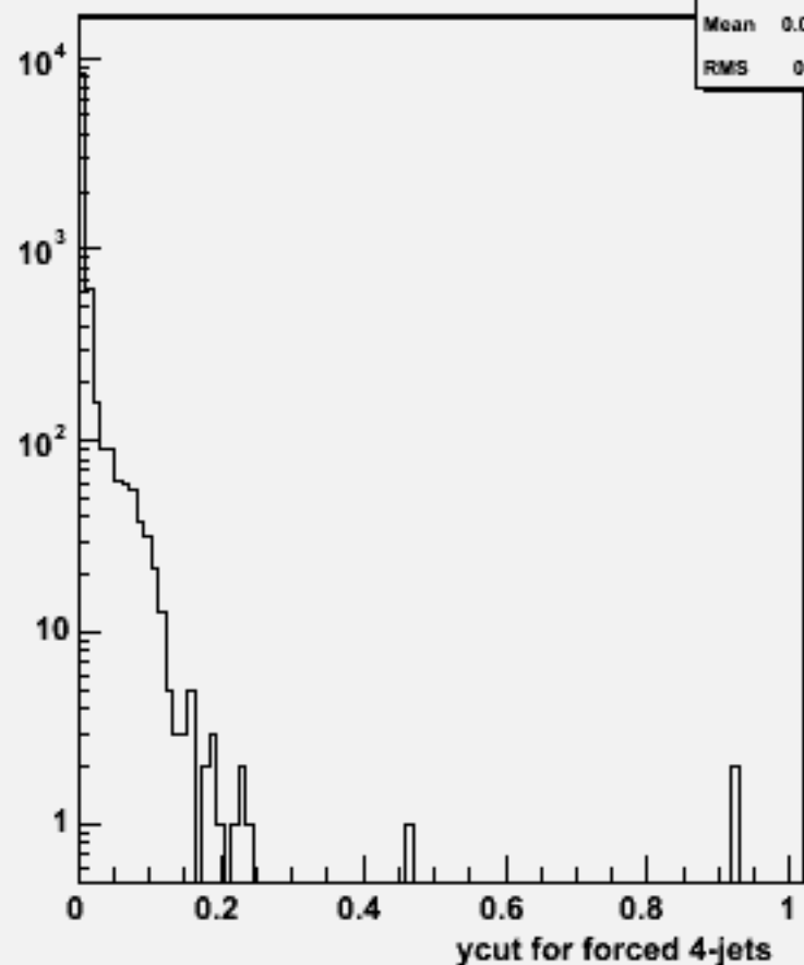
Ycut for 4-jets :w103327 e1a_e1uubb_o
