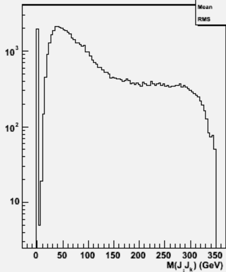
2jets mass(All comb)w103327 e1a_e1uubb_o
