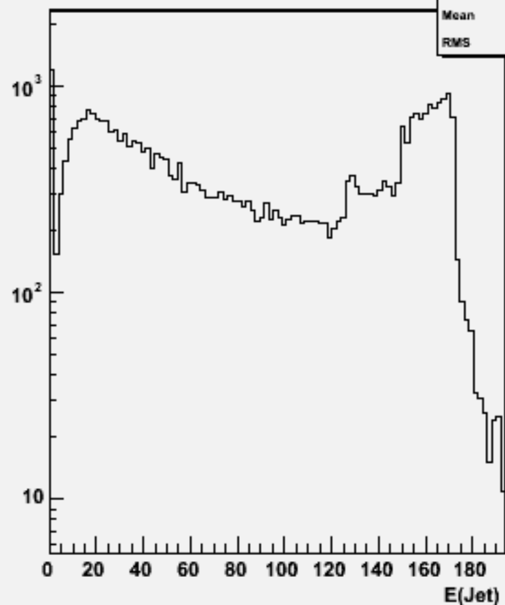
Jet energies(All jets)w103327 e1a_e1uubb_o
