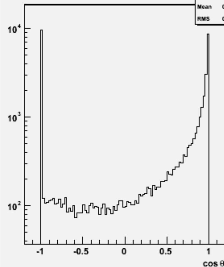
Jet cos \theta (All jets)w103327 e1a_e1uubb_o
