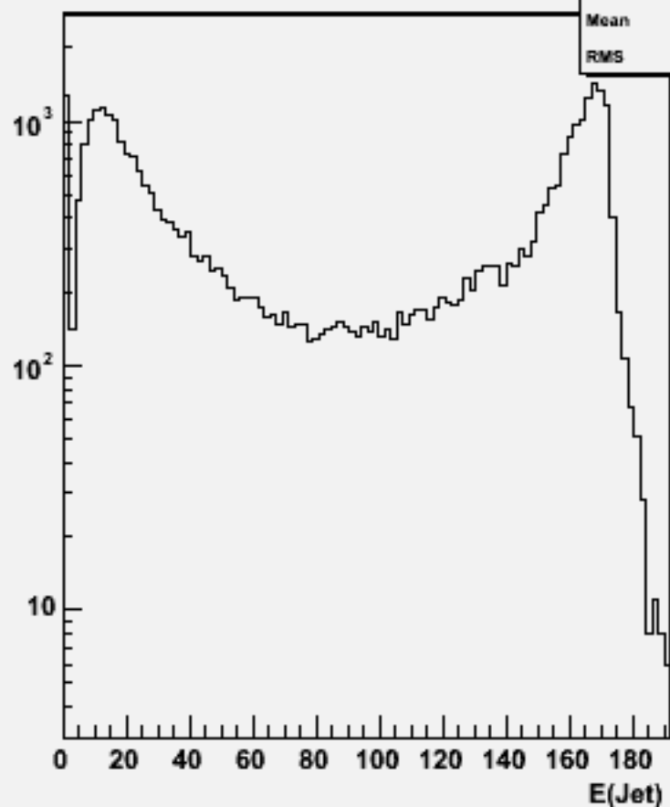
Jet energies(All jets)w103311 e1a_e1uue1e1_o
