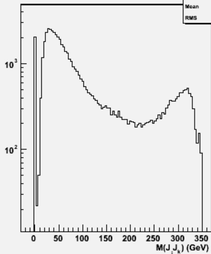
2jets mass(All comb)w103311 e1a_e1uue1e1_o
