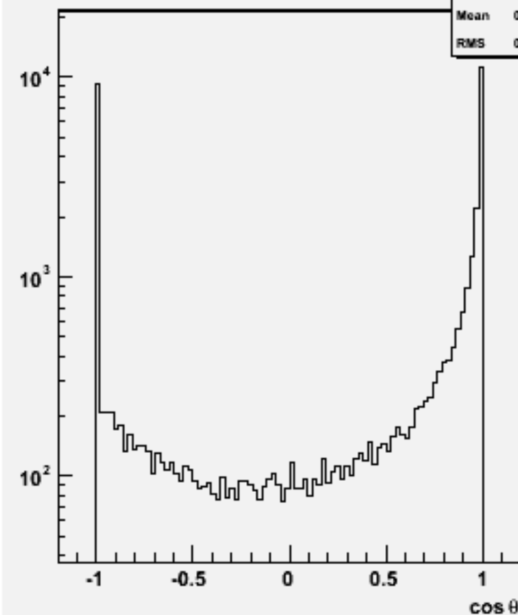
Jet cos \theta (All jets)w103311 e1a_e1uue1e1_o
