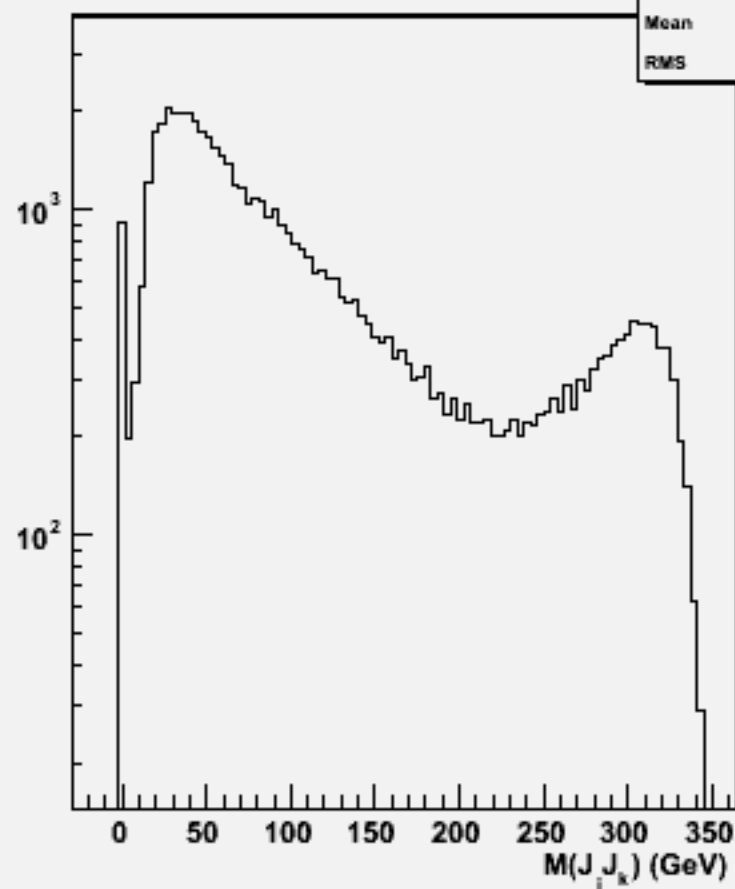
2jets mass(All comb)w103310 e1a_e1uue1e1_o
