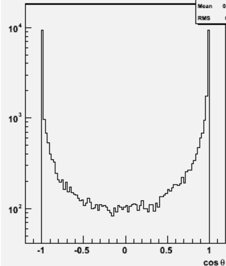
Jet cos \theta (All jets)w103310 e1a_e1uue1e1_o
