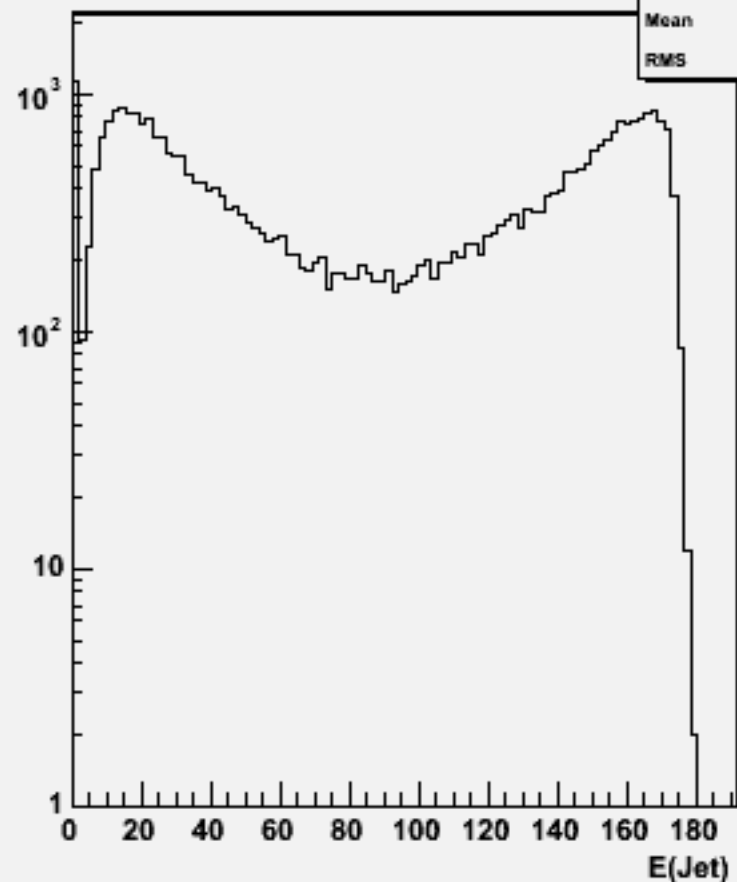
Jet energies(All jets)w103310 e1a_e1uue1e1_o
