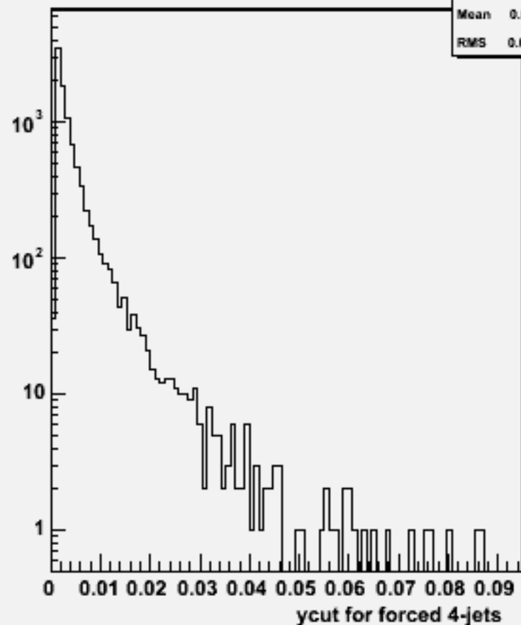
Ycut for 4-jets :w103310 e1a_e1uue1e1_o
