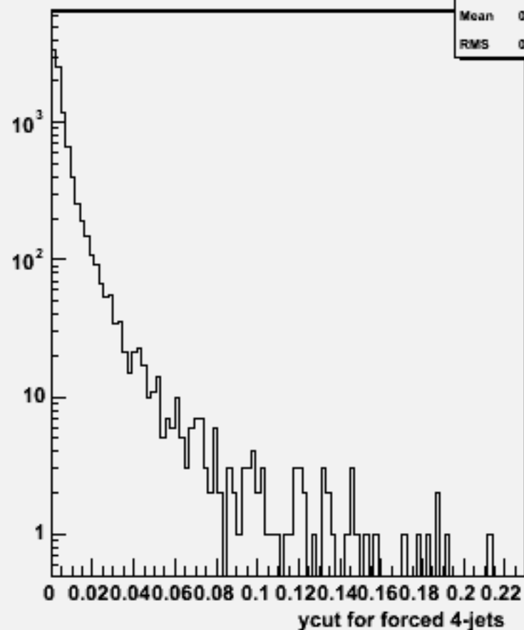
Ycut for 4-jets :w103302 e1a_e1n3n3ss_o
