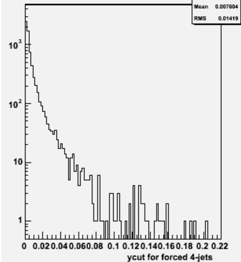
Ycut for 4-jets :w103292 e1a_e1n3n3e1e1_o
