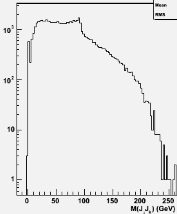
2jets mass(All comb)w103286 e1a_e1n2n2bb_o
