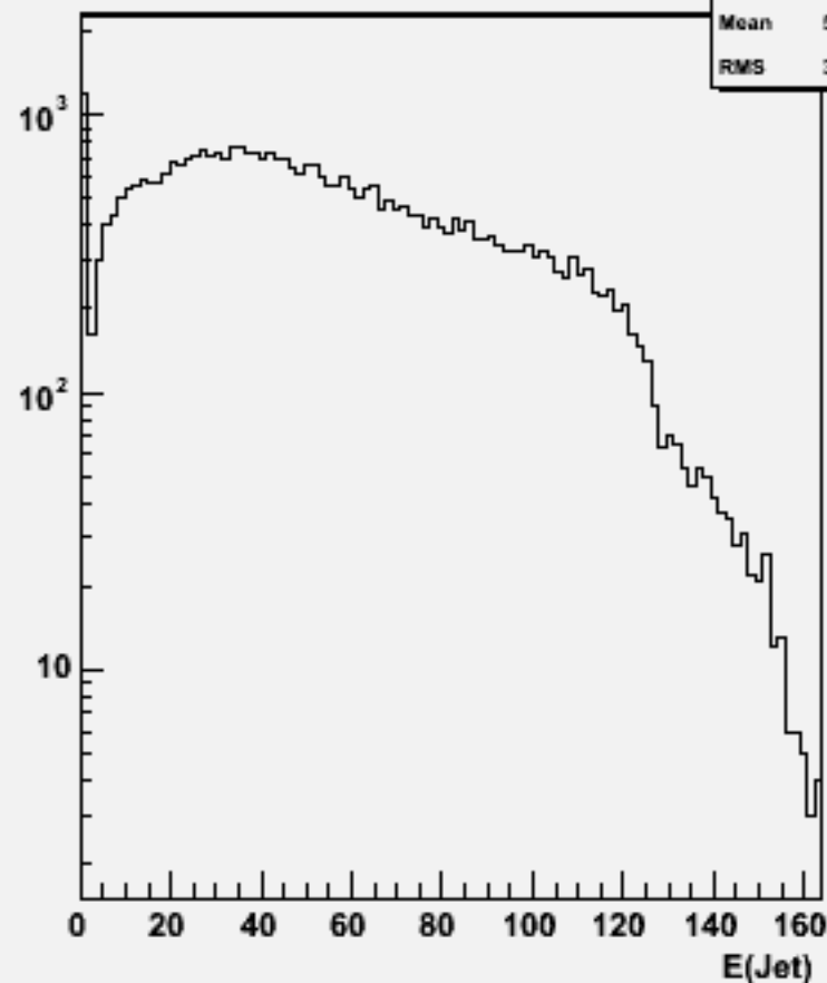
Jet energies(All jets)w103286 e1a_e1n2n2bb_o
