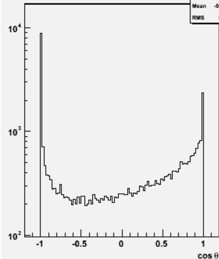
Jet cos \theta (All jets)w103286 e1a_e1n2n2bb_o
