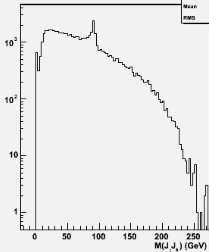
2jets mass(All comb)w103284 e1a_e1n2n2ss_o
