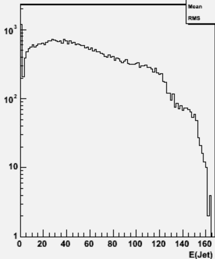
Jet energies(All jets)w103284 e1a_e1n2n2ss_o
