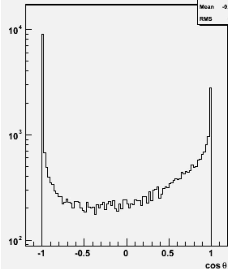
Jet cos \theta (All jets)w103284 e1a_e1n2n2ss_o
