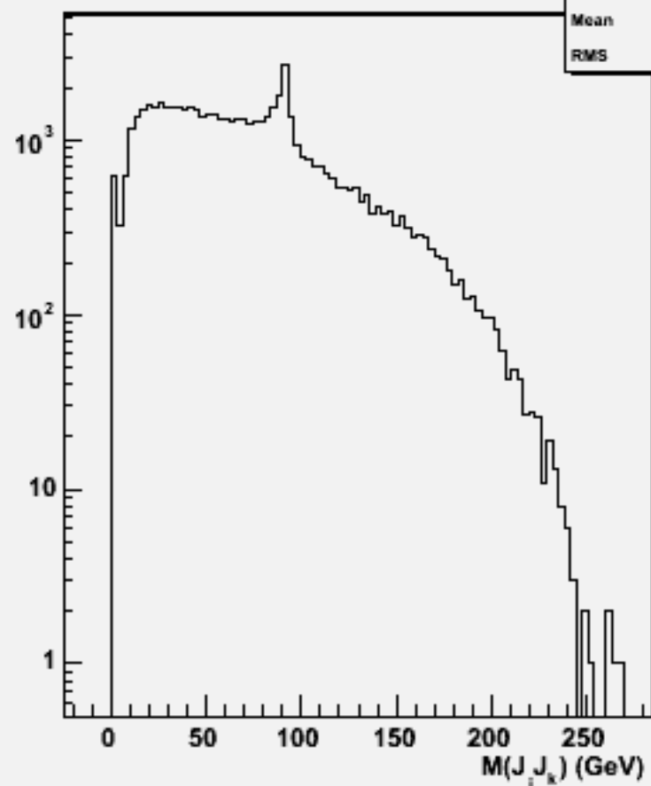
2jets mass(All comb)w103282 e1a_e1n2n2ss_o
