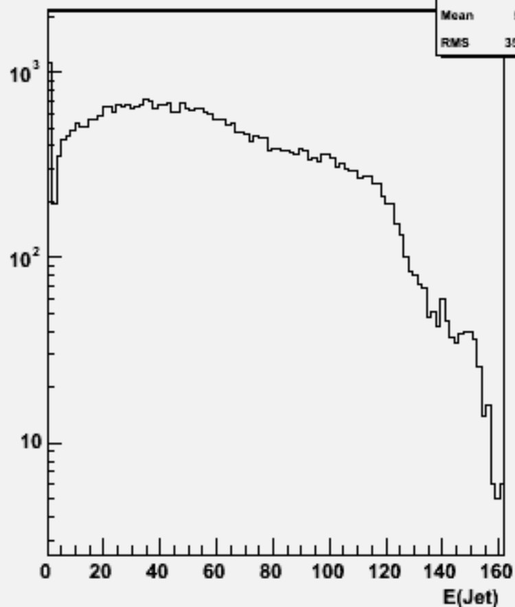
Jet energies(All jets)w103282 e1a_e1n2n2ss_o
