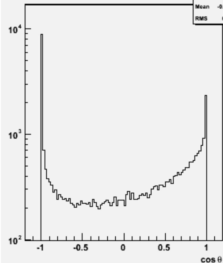
Jet cos \theta (All jets)w103282 e1a_e1n2n2ss_o
