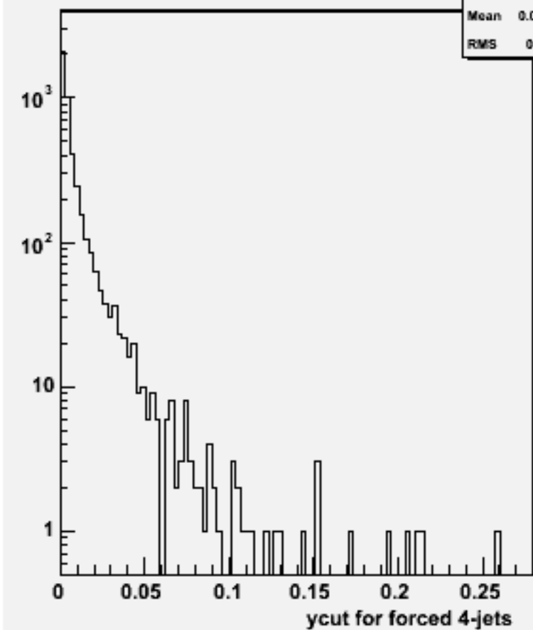
Ycut for 4-jets :w103276 e1a_e1n2n2e3e3_o
