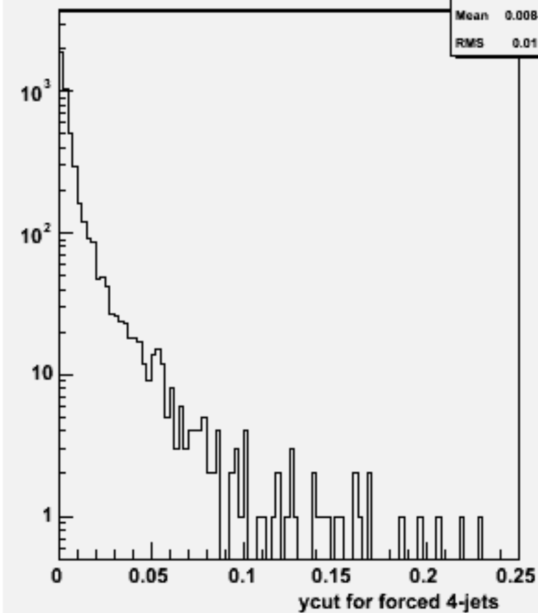
Ycut for 4-jets :w103274 e1a_e1n2n2e3e3_o
