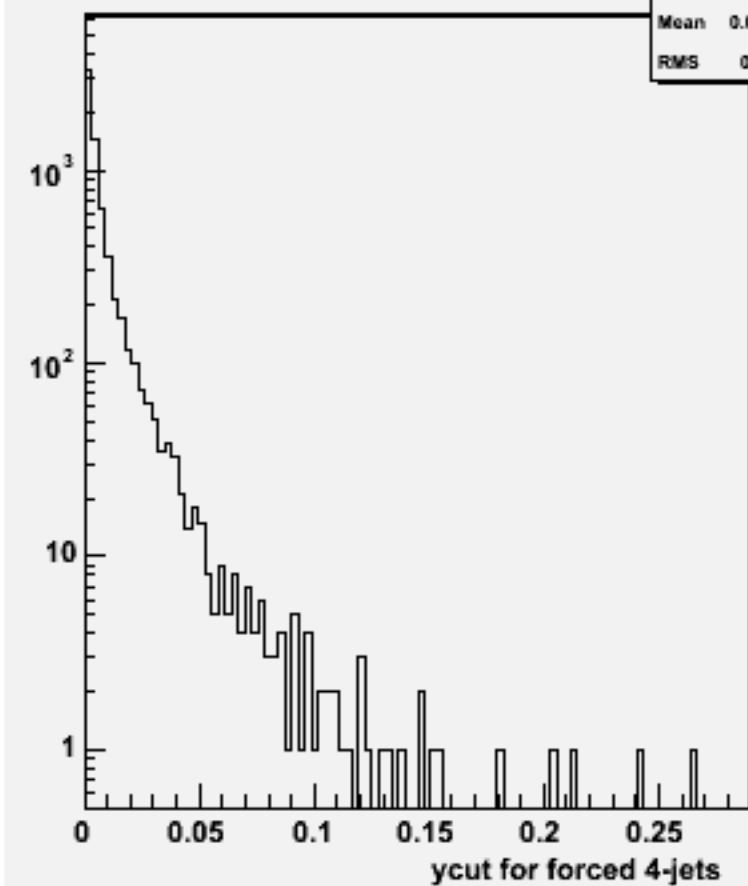
Ycut for 4-jets :w103272 e1a_e1n2n2e1e1_o
