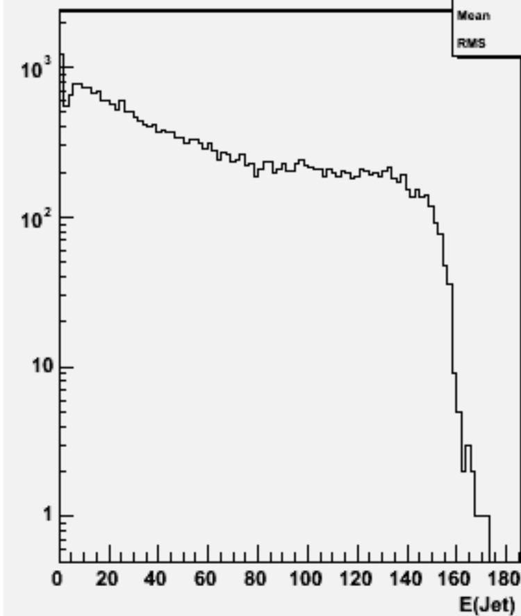
Jet energies(All jets)w103272 e1a_e1n2n2e1e1_o
