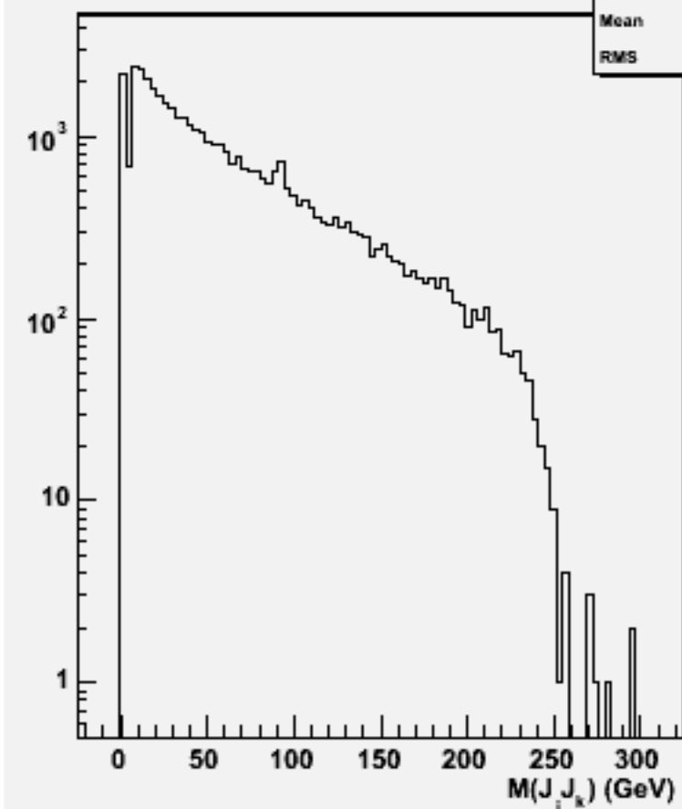
2jets mass(All comb)w103272 e1a_e1n2n2e1e1_o
