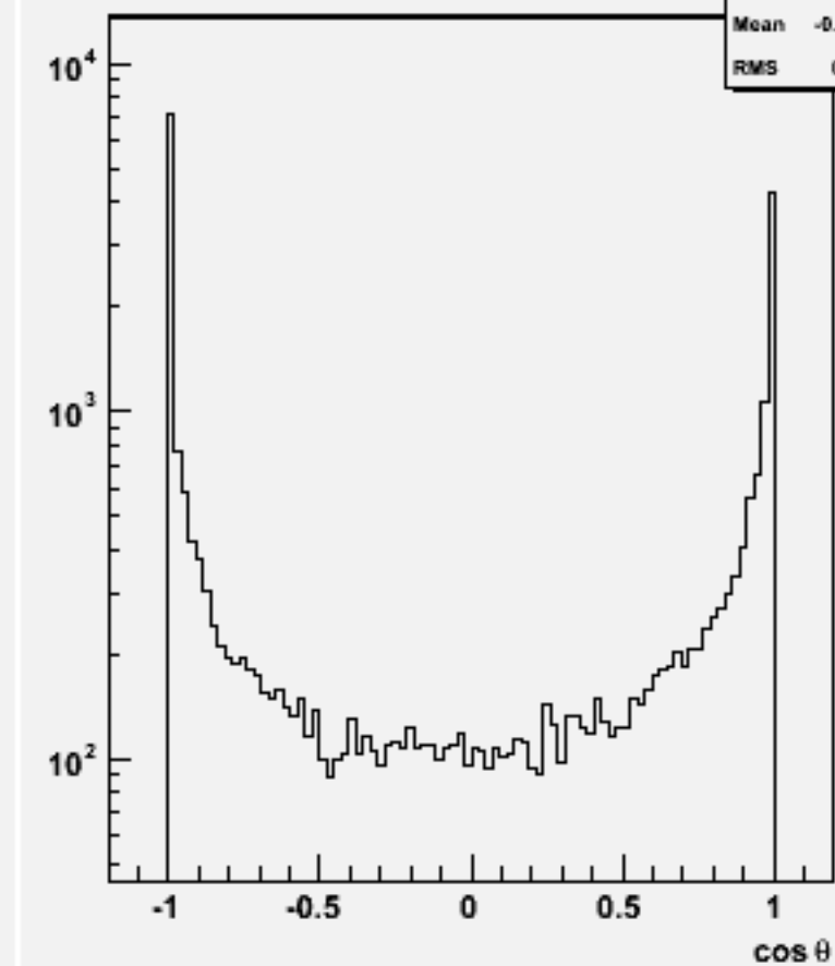
Jet cos \theta (All jets)w103272 e1a_e1n2n2e1e1_o
