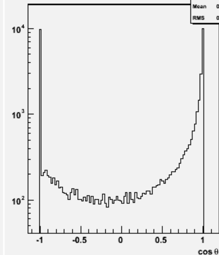
Jet cos \theta (All jets)w103269 e1a_e1cccc_o
