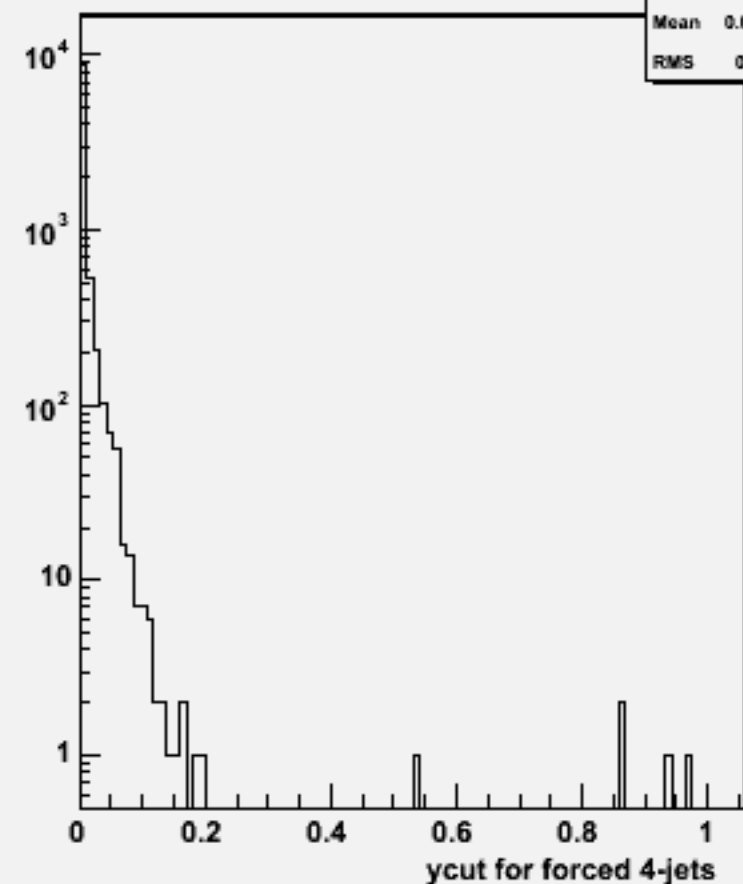
Ycut for 4-jets :w103269 e1a_e1cccc_o
