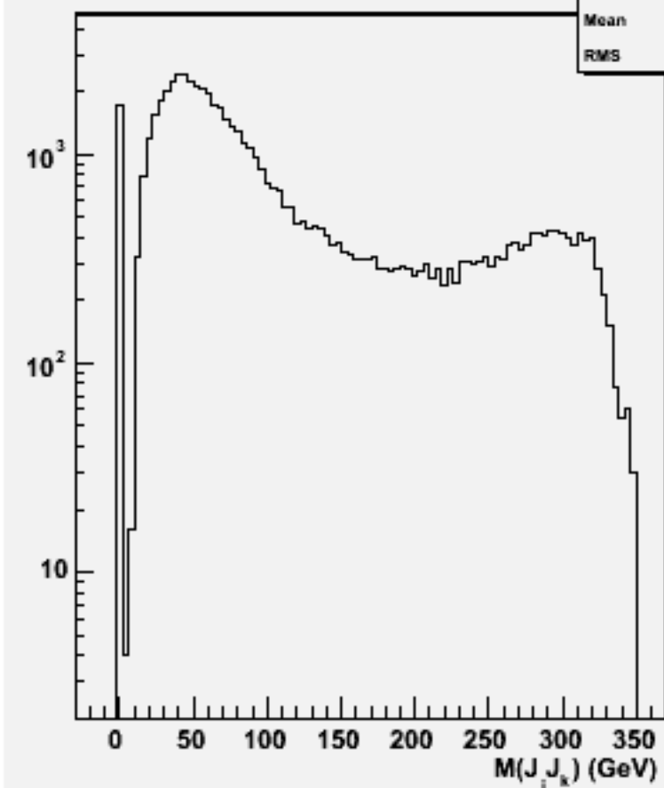
2jets mass(All comb)w103269 e1a_e1cccc_o
