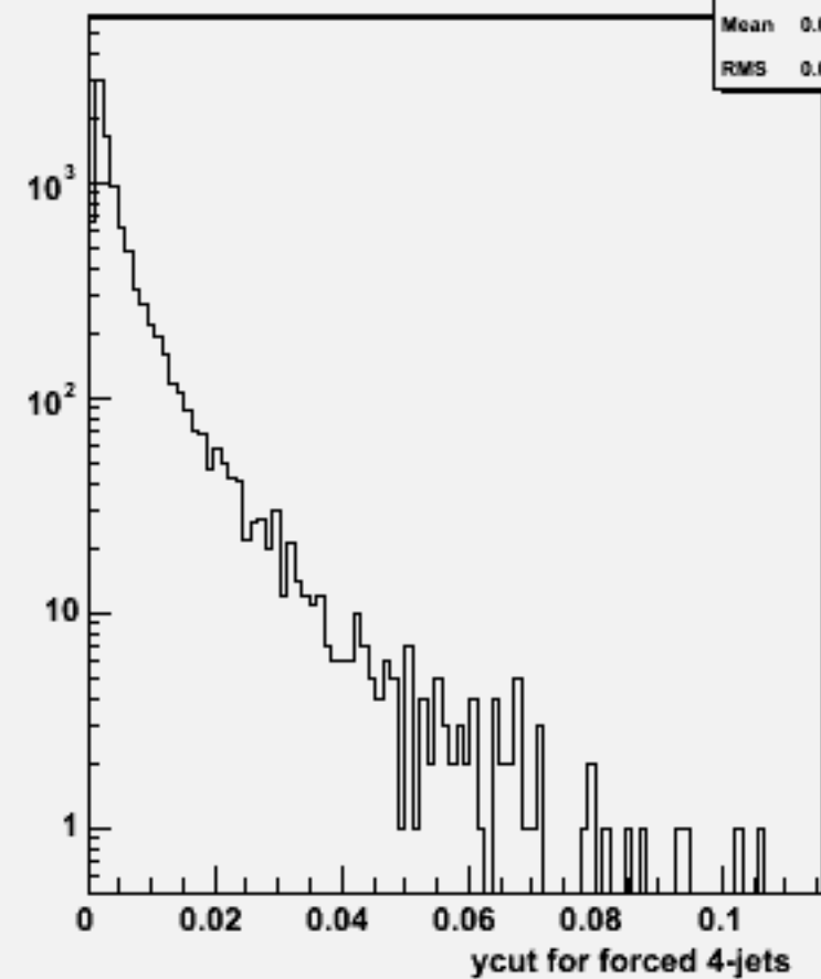
Ycut for 4-jets :w103268 e1a_e1cccc_o
