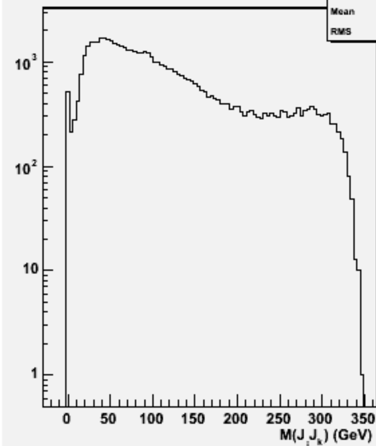
2jets mass(All comb)w103268 e1a_e1cccc_o
