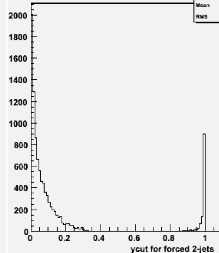
Ycut for 2-jets :w103266 e1a_e1cccc_o
