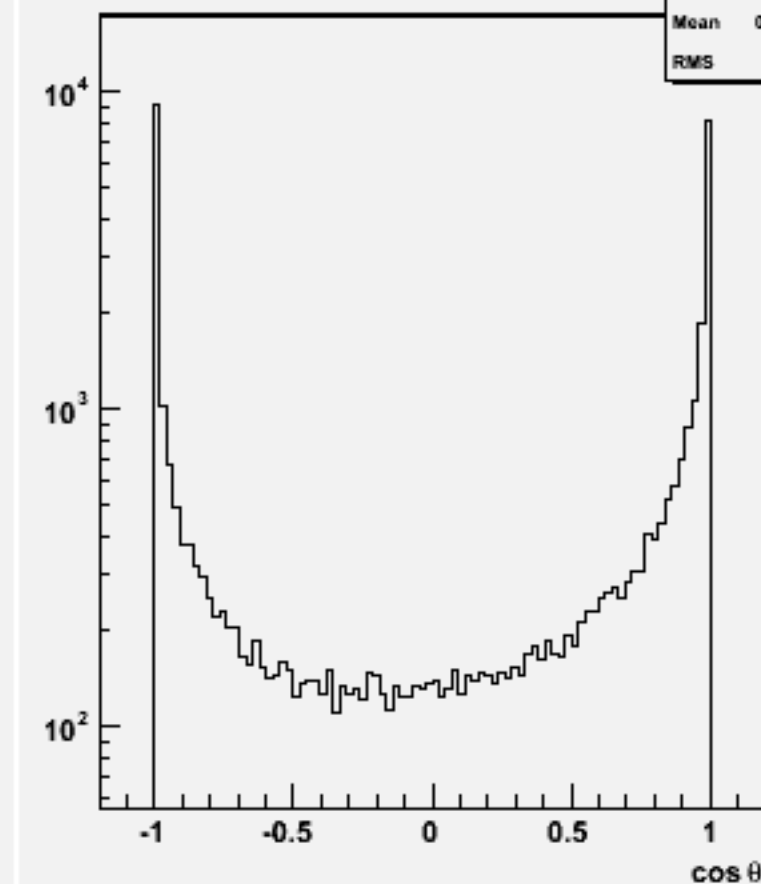
Jet cos \theta (All jets)w103266 e1a_e1cccc_o
