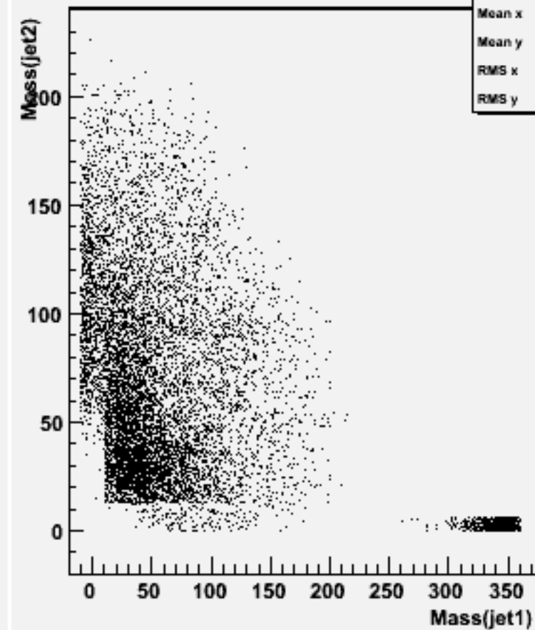
Jet mass for forced 2-jets : w103266 e1a_e1cccc_o
