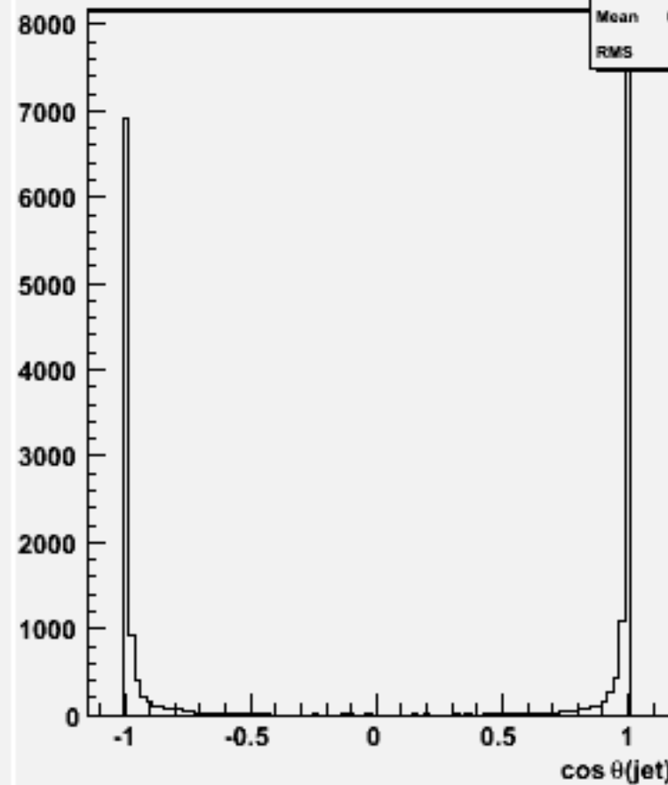
cos \theta for 2-jets :w103266 e1a_e1cccc_o
