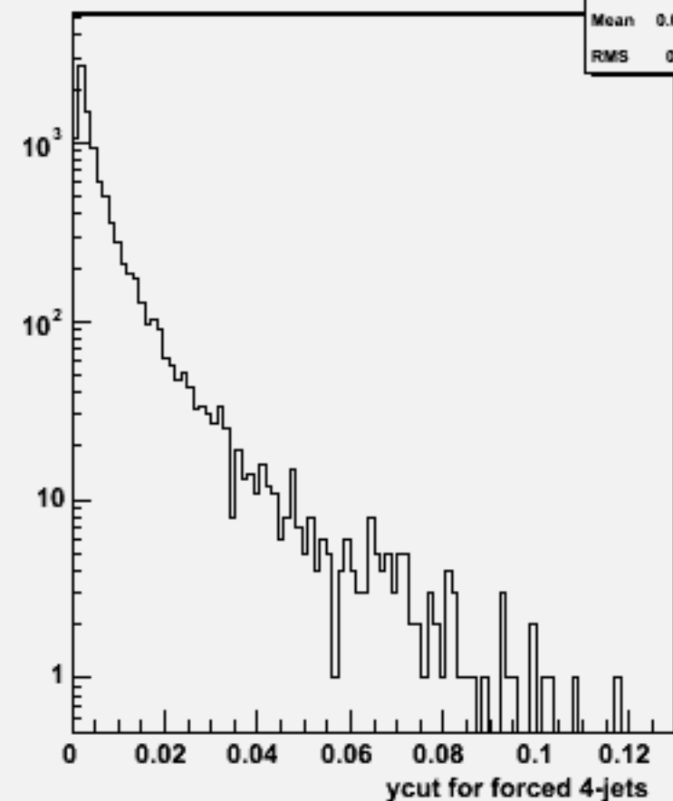
Ycut for 4-jets :w103266 e1a_e1cccc_o
