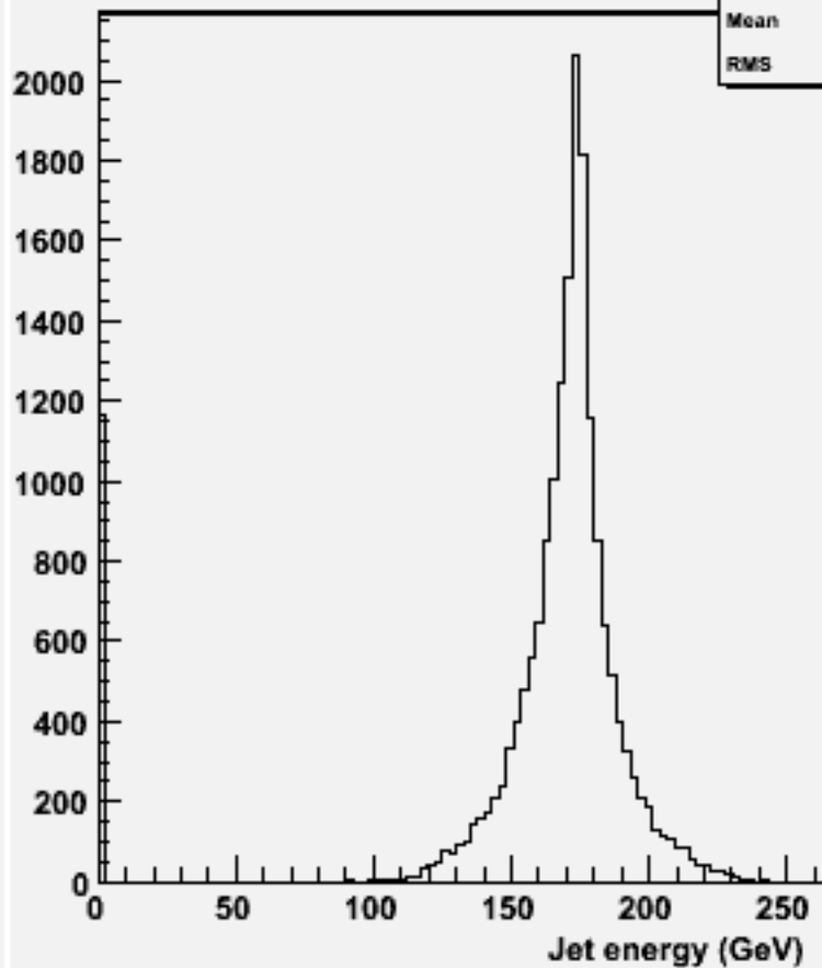
energy for 2-jets :w103266 e1a_e1cccc_o
