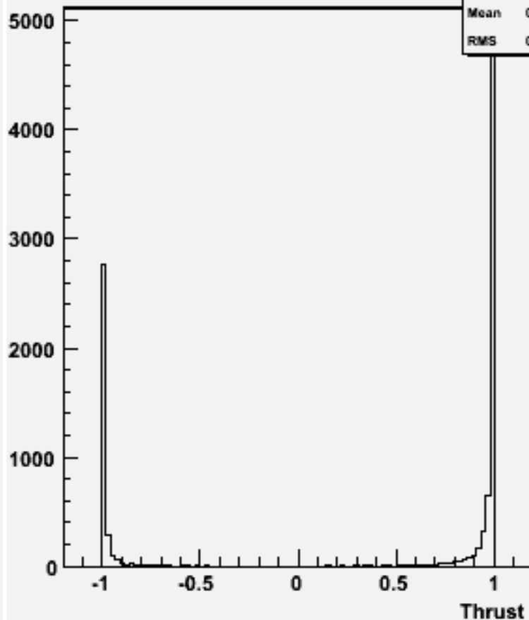
cos \Theta (thrust) w103266 e1a_e1cccc_o
