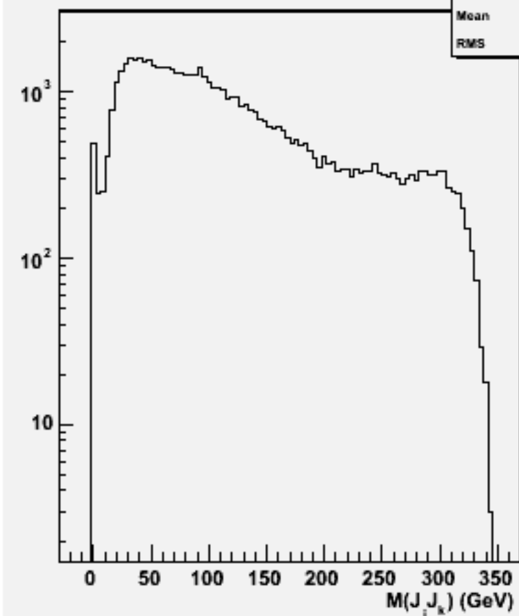
2jets mass(All comb)w103266 e1a_e1cccc_o
