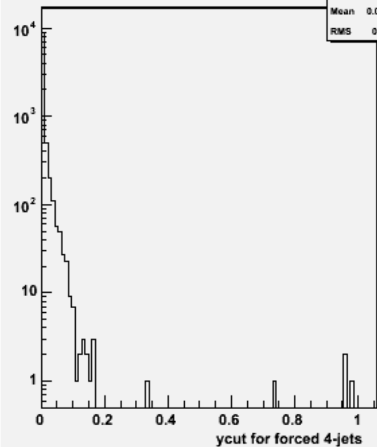
Ycut for 4-jets :w103265 e1a_e1uucc_o
