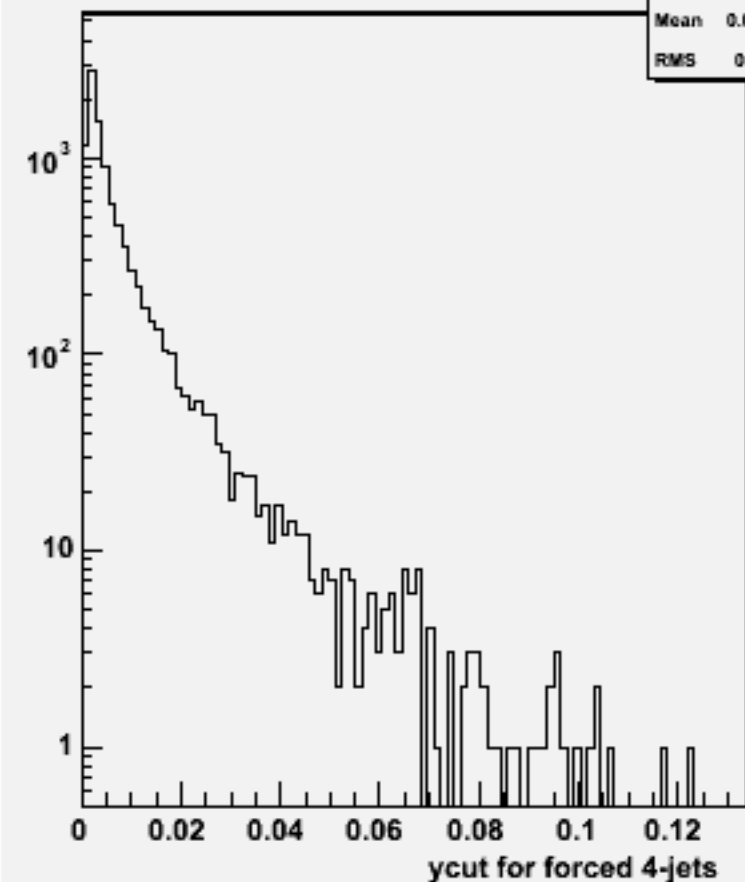
Ycut for 4-jets :w103262 e1a_e1uucc_o
