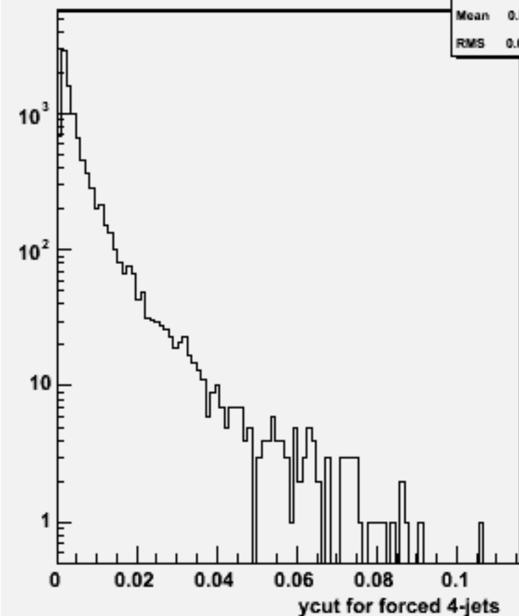
Ycut for 4-jets :w103260 e1a_e1uuuu_o
