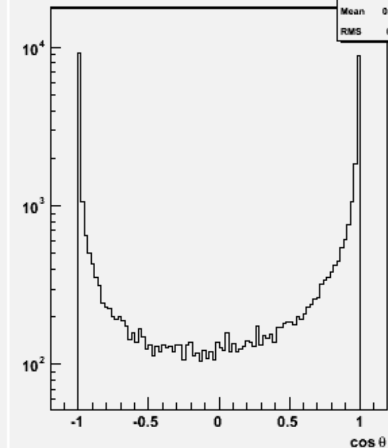
Jet cos \theta (All jets)w103260 e1a_e1uuuu_o
