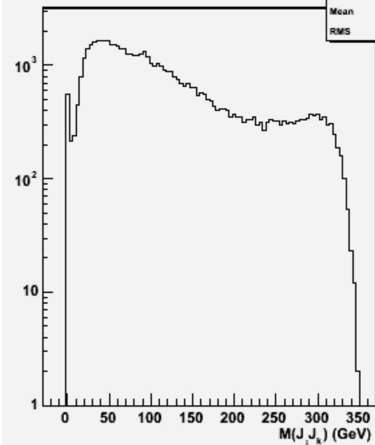
2jets mass(All comb)w103260 e1a_e1uuuu_o
