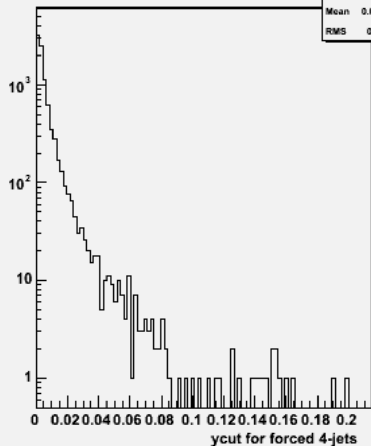
Ycut for 4-jets :w103254 e1a_e1n3n3cc_o
