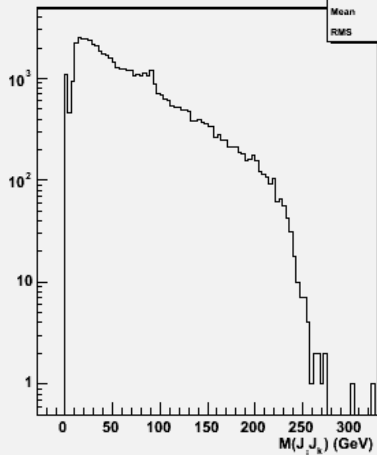
2jets mass(All comb)w103244 e1a_e1n2n2cc_o
