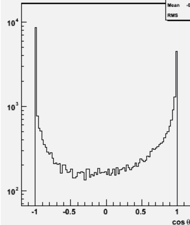
Jet cos \theta (All jets)w103244 e1a_e1n2n2cc_o
