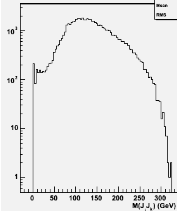
2jets mass(All comb)w103226 e1a_e1cssc_o
