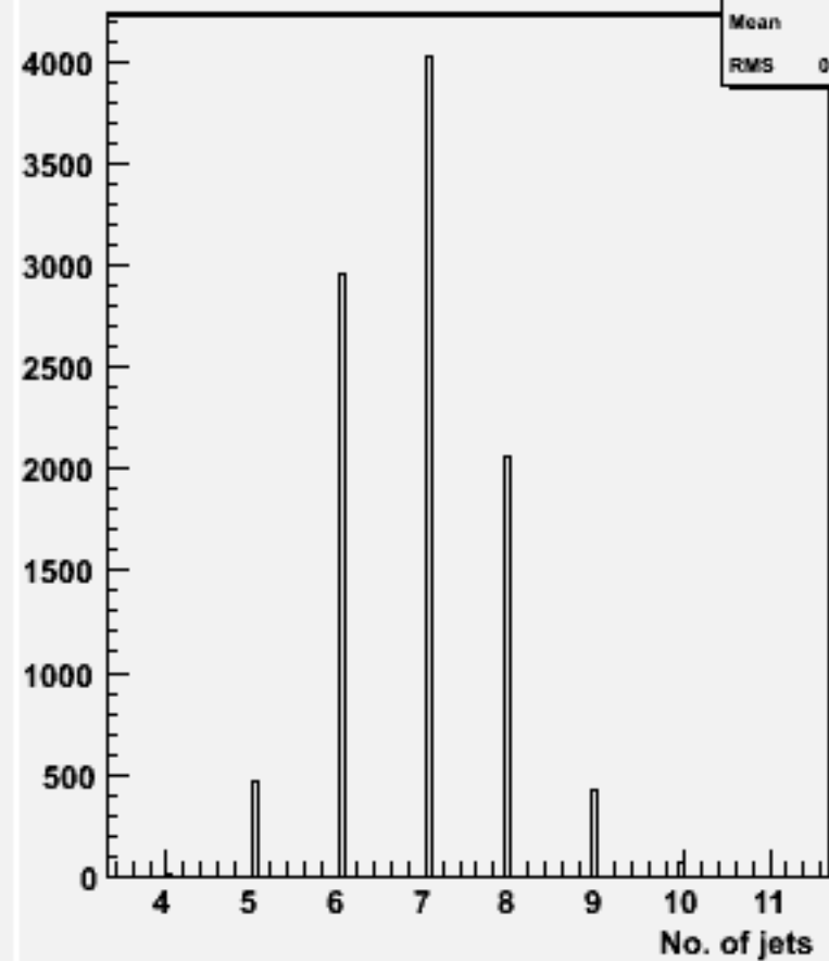
No. jets (ycut=0.001) : w103226 e1a_e1cssc_o
