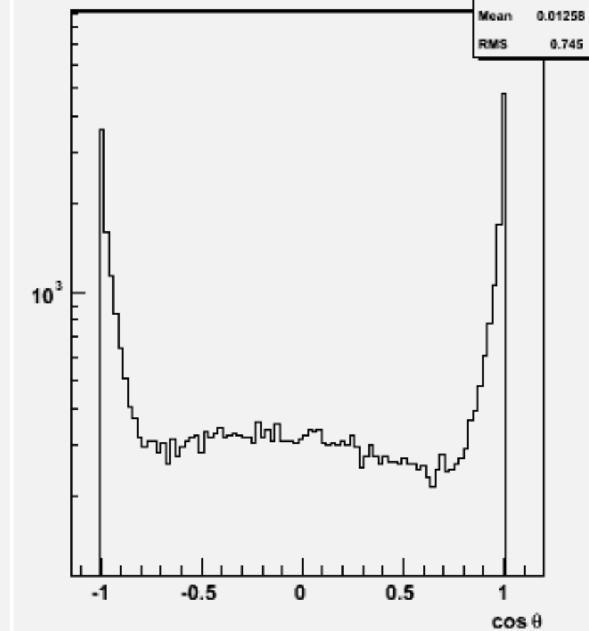
Jet cos \theta (All jets)w103226 e1a_e1cssc_o
