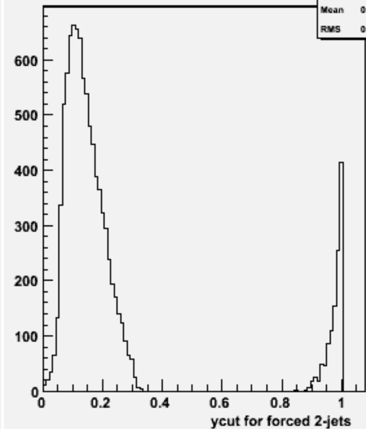
Ycut for 2-jets :w103226 e1a_e1cssc_o
