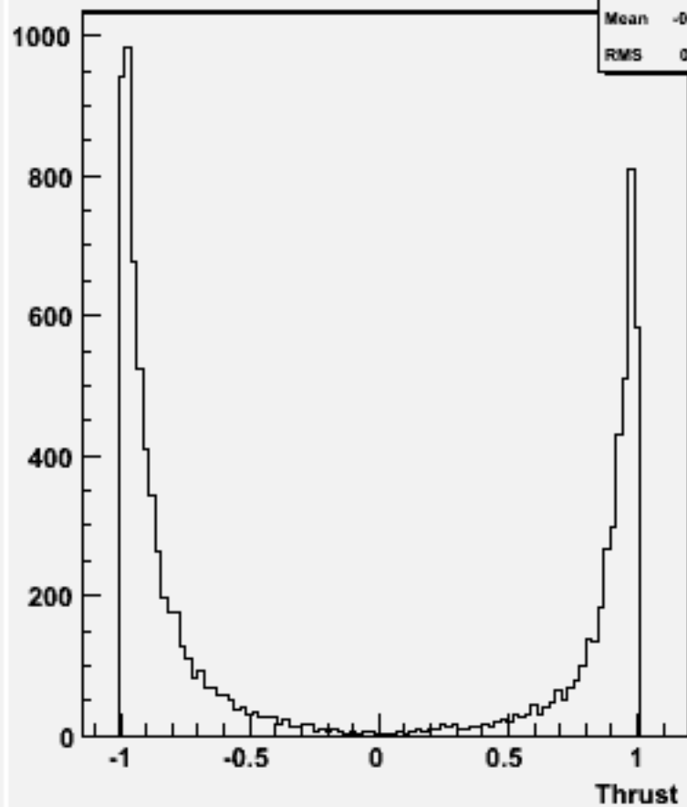
cos \Theta (thrust) w103226 e1a_e1cssc_o
