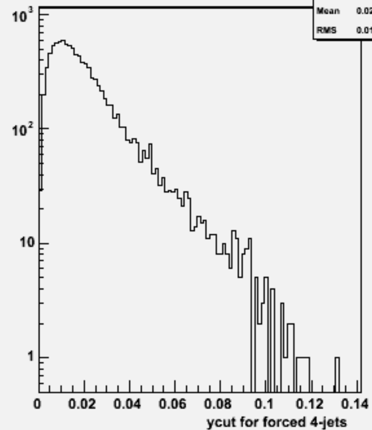
Ycut for 4-jets :w103226 e1a_e1cssc_o
