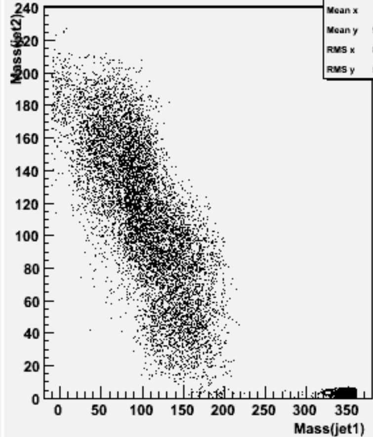
Jet mass for forced 2-jets : w103226 e1a_e1cssc_o
