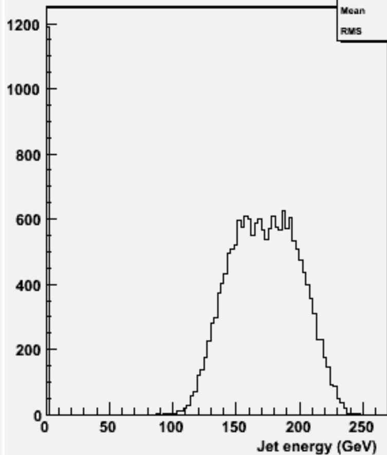
energy for 2-jets :w103226 e1a_e1cssc_o
