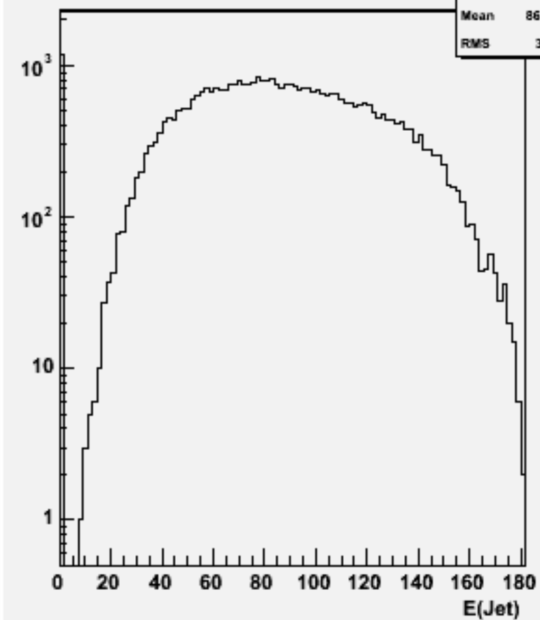
Jet energies(All jets)w103226 e1a_e1cssc_o
