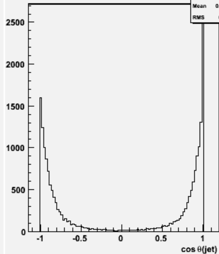
cos \theta for 2-jets :w103226 e1a_e1cssc_o
