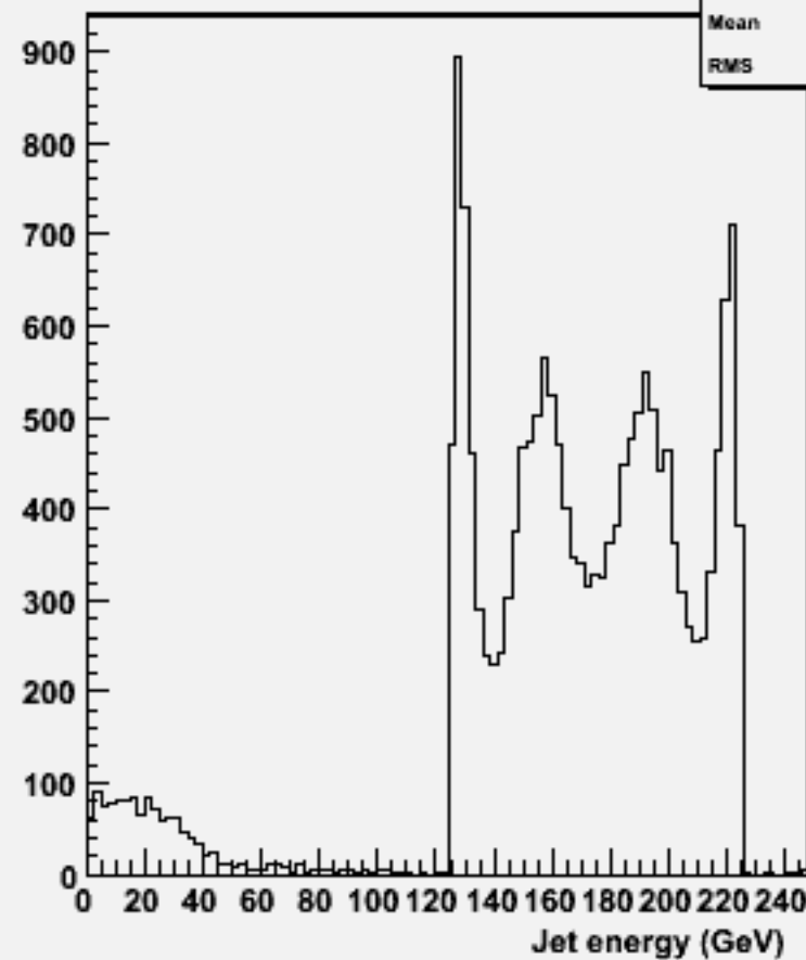
energy for 2-jets :w103225 e1a_e1csdu_o
