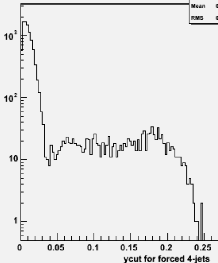
Ycut for 4-jets :w103225 e1a_e1csdu_o
