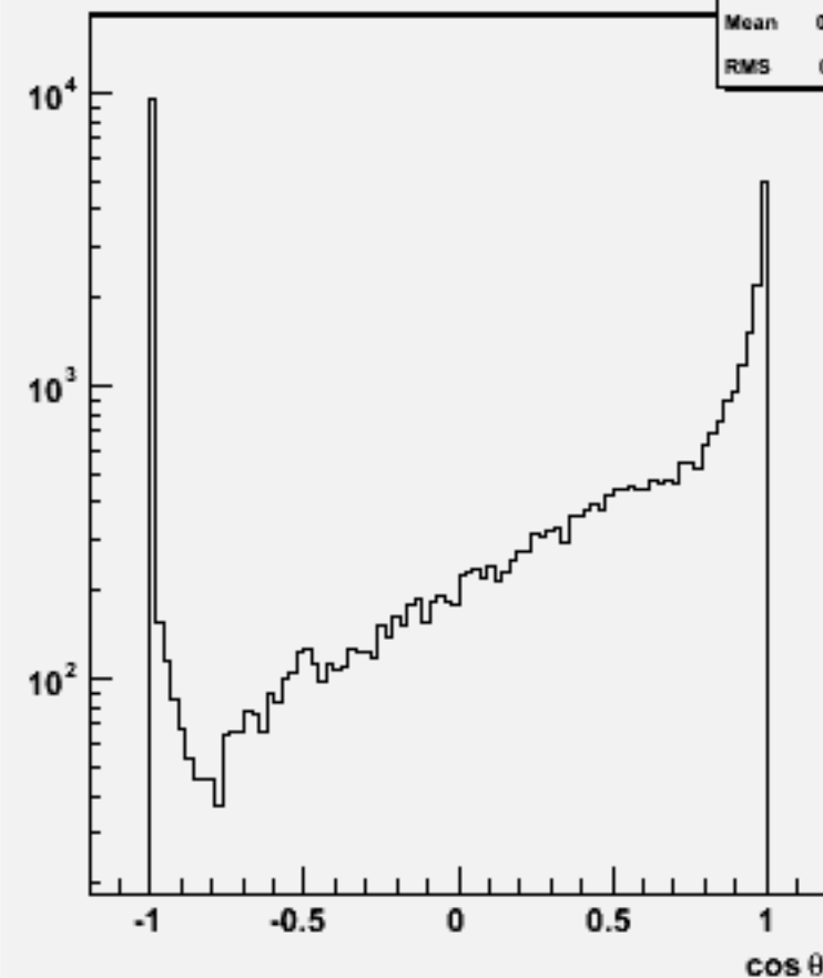
Jet cos \theta (All jets)w103225 e1a_e1csdu_o
