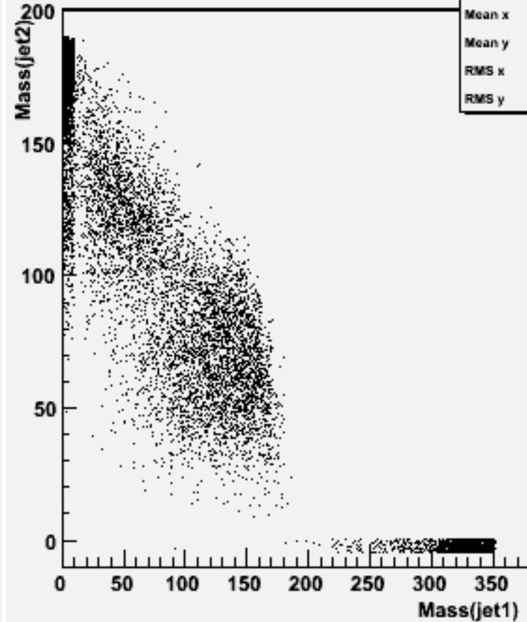
Jet mass for forced 2-jets : w103225 e1a_e1csdu_o
