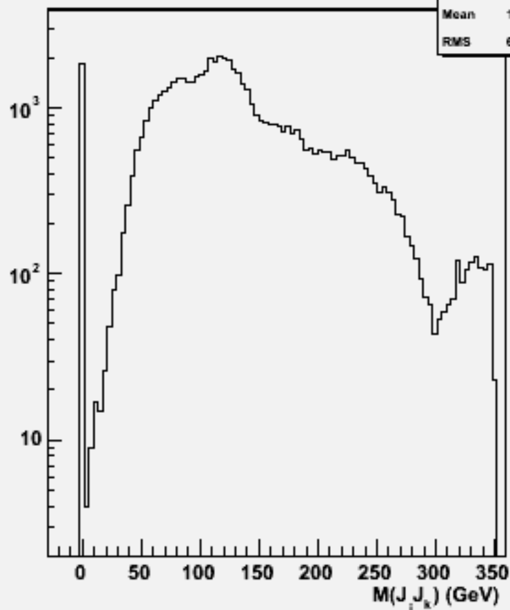
2jets mass(All comb)w103225 e1a_e1csdu_o
