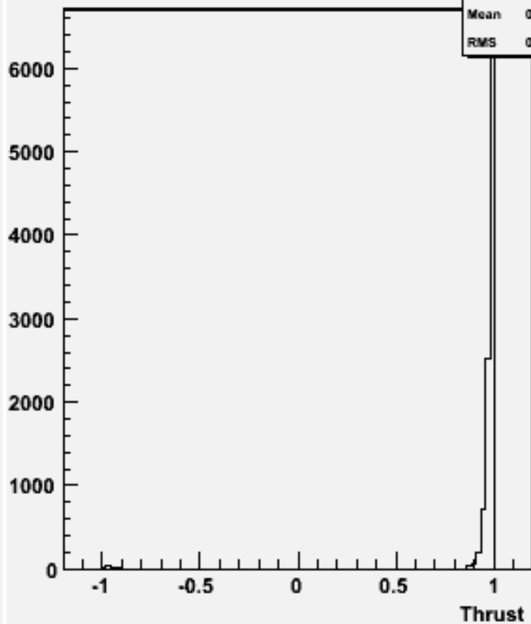
cos \Theta (thrust) w103225 e1a_e1csdu_o
