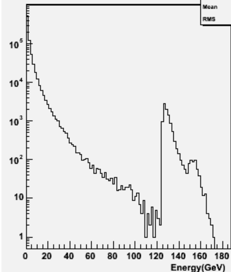
Particle Energy : w103225 e1a_e1csdu_o
