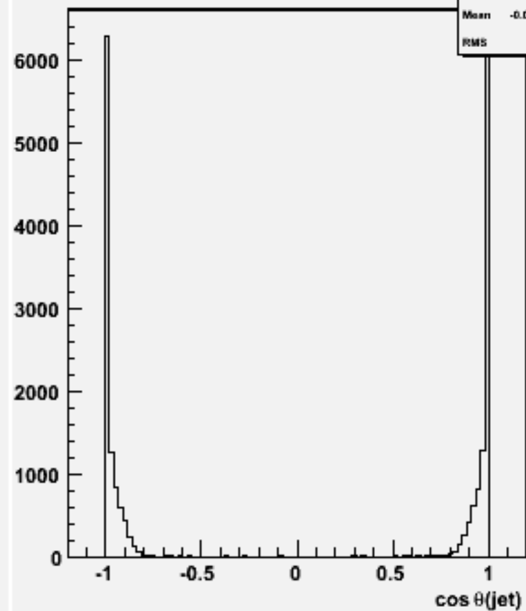
cos \theta for 2-jets :w103225 e1a_e1csdu_o
