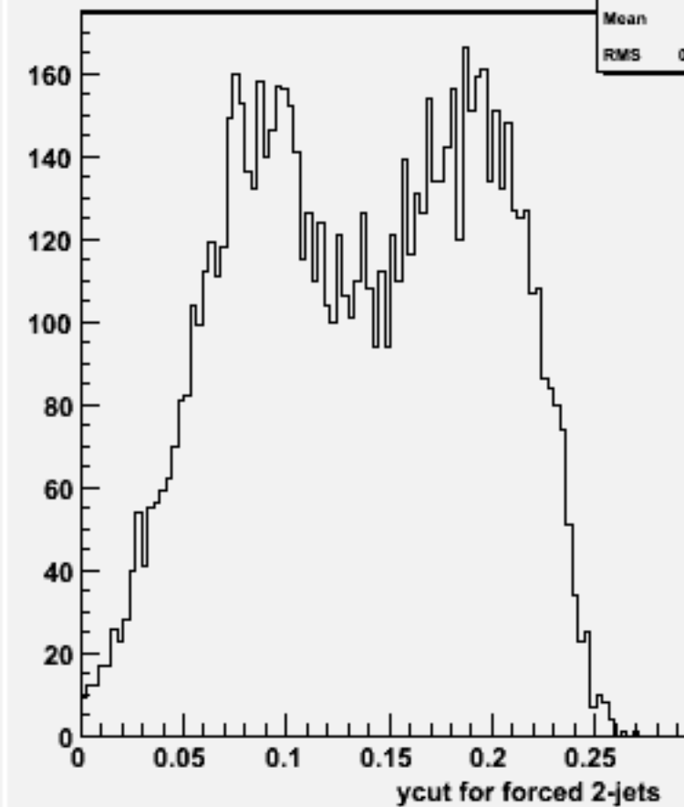
Ycut for 2-jets :w103225 e1a_e1csdu_o
